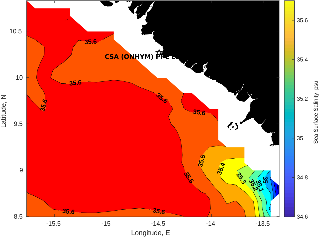
Surface Salinity for CSA (ONHYM) PPL EBS - Guinea at 21-May-2025 00:00:00
