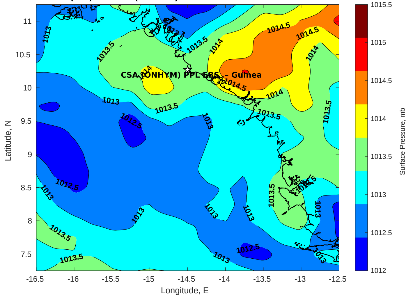
Surface Pressure (mb) for CSA (ONHYM) PPL EBS - Guinea at 15-Nov-2030 00:00:00
