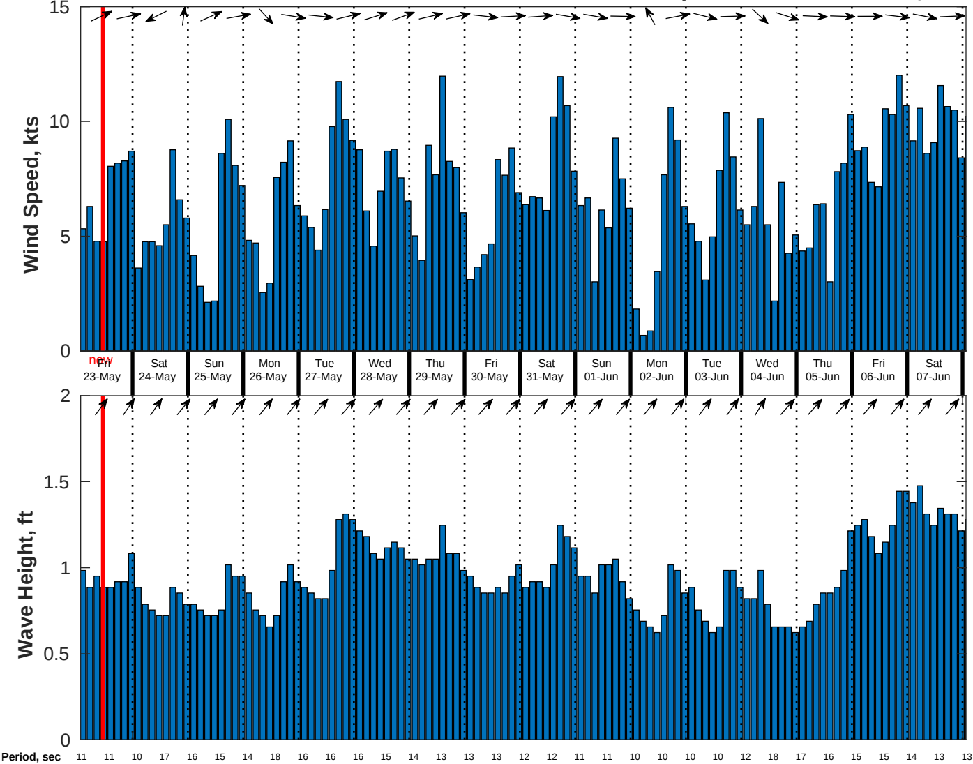
Wind & Wave Forecast for CSA (ONHYM) PPL EBS - Guinea from 22-May-2025 01:00:00 to 07-Jun-2025 01:00:00
