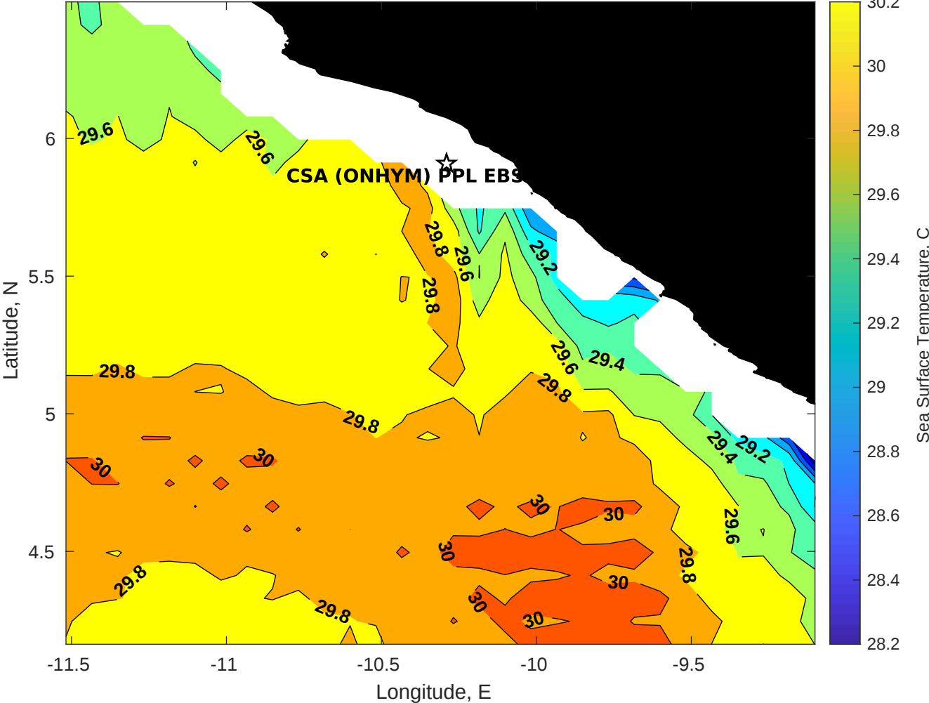
SST for CSA (ONHYM) PPL EBS - Liberia at 21-May-2025 00:00:00
