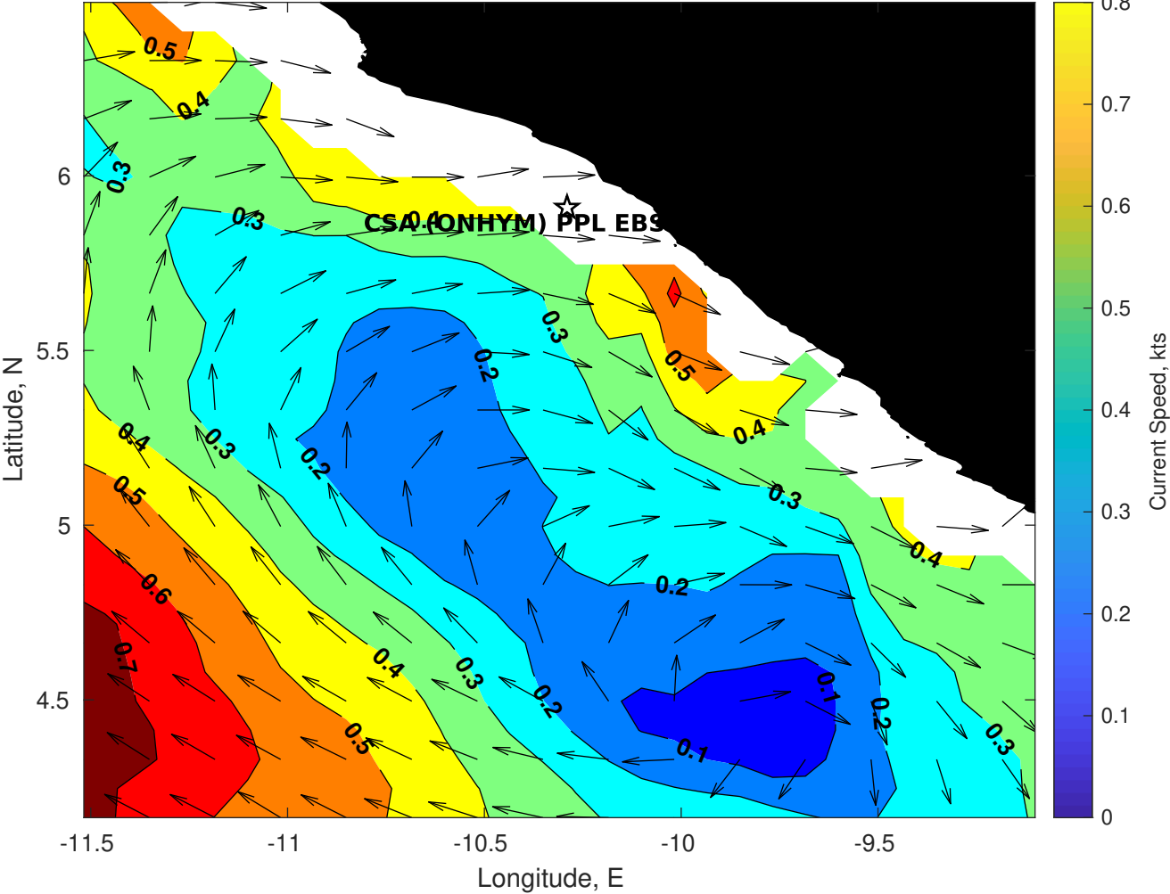
Surface Currents for CSA (ONHYM) PPL EBS - Liberia at 21-May-2025 00:00:00
