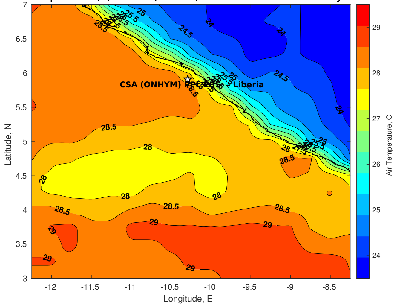
Air Temperature (C) for CSA (ONHYM) PPL EBS - Liberia at 22-May-2025
