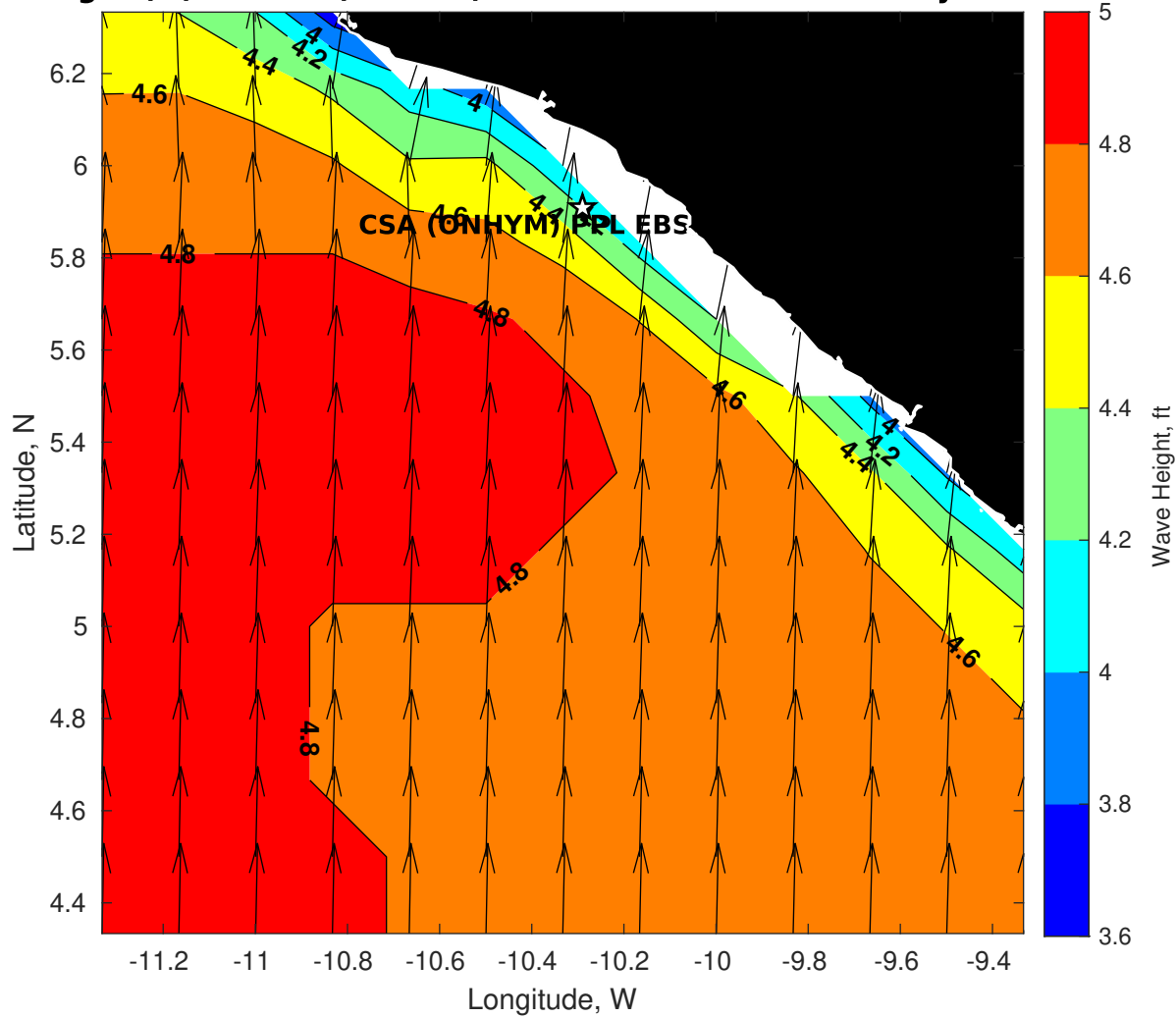
Wave Height (ft) for CSA (ONHYM) PPL EBS - Liberia at 22-May-2025 09:00:00
