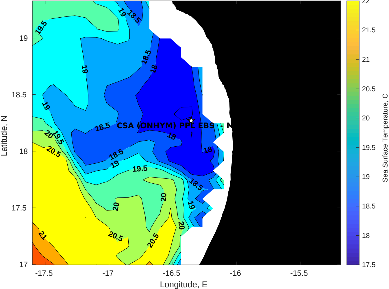
SST for CSA (ONHYM) PPL EBS - Mauritania at 21-May-2025 00:00:00
