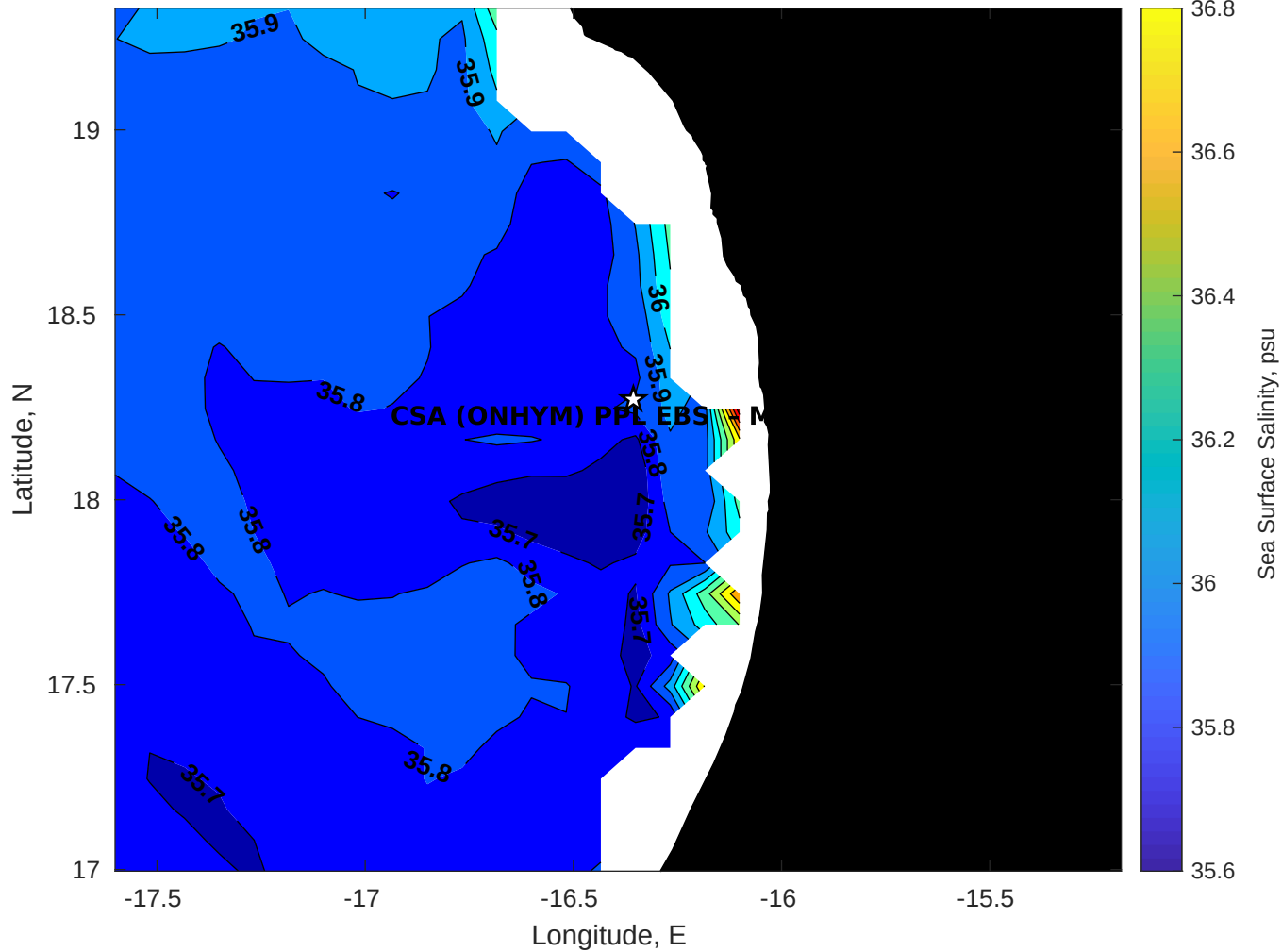
Surface Salinity for CSA (ONHYM) PPL EBS - Mauritania at 21-May-2025 00:00:00
