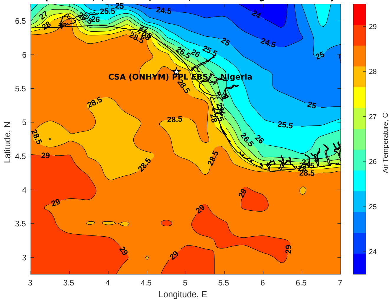
Air Temperature (C) for CSA (ONHYM) PPL EBS - Nigeria at 22-May-2025
