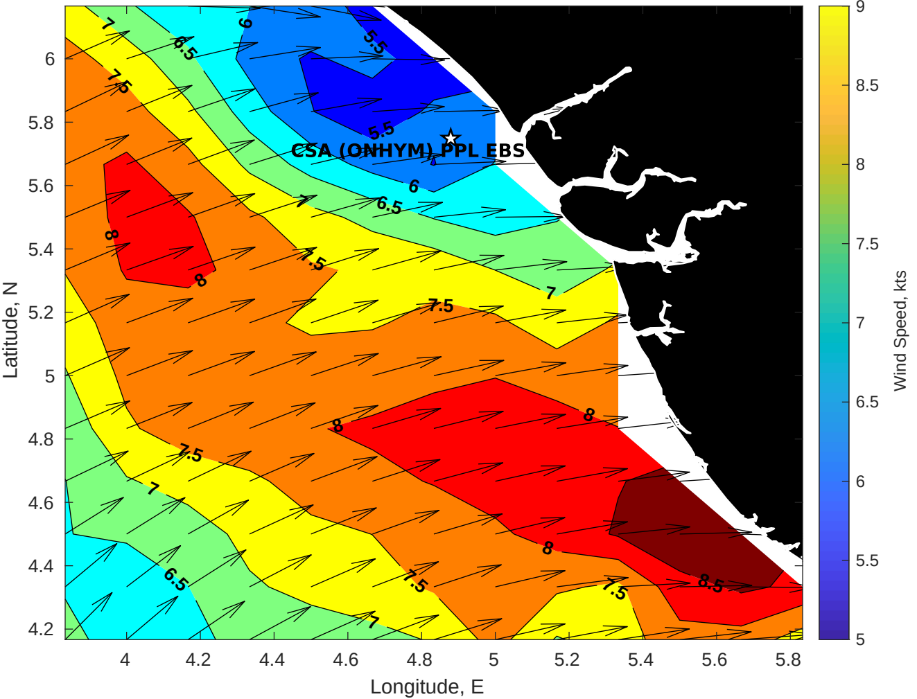
Winds (kts) for CSA (ONHYM) PPL EBS - Nigeria at 22-May-2025 09:00:00
