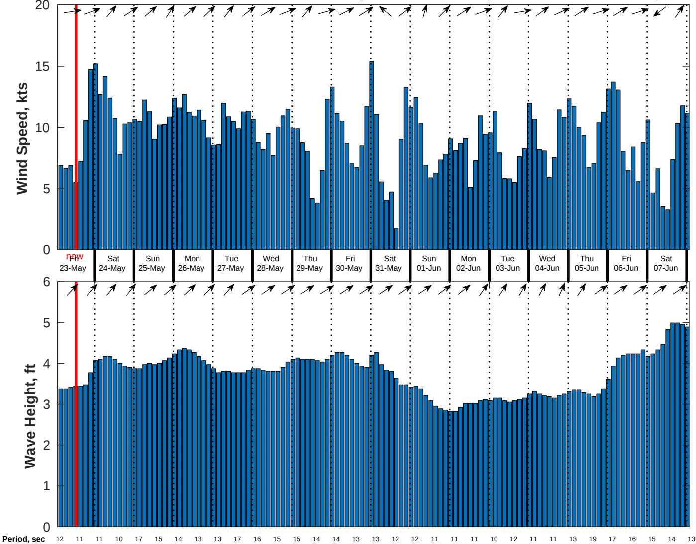
Wind & Wave Forecast for CSA (ONHYM) PPL EBS - Nigeria from 22-May-2025 02:00:00 to 07-Jun-2025 02:00:00
