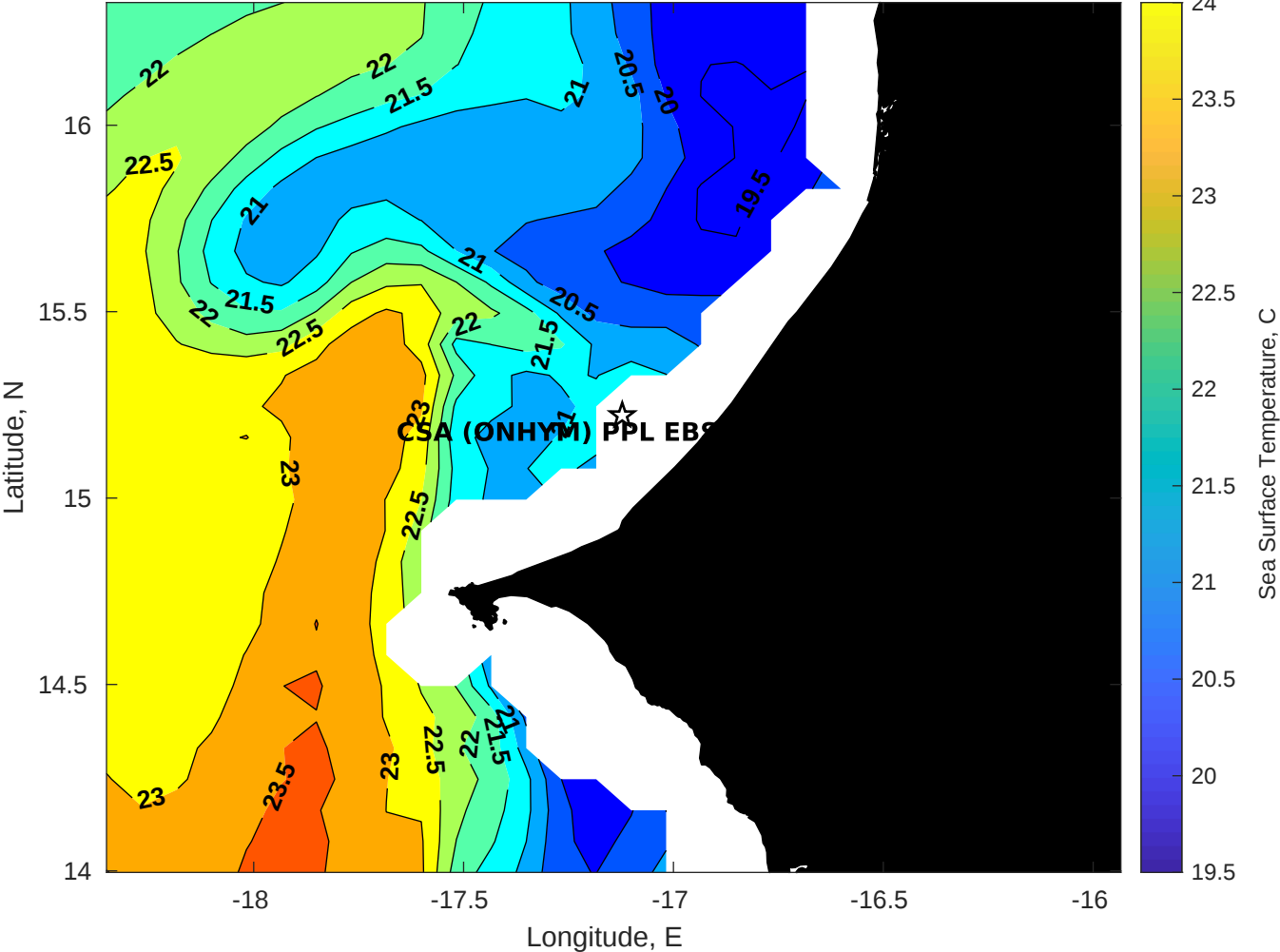
SST for CSA (ONHYM) PPL EBS - Senegal at 21-May-2025 00:00:00
