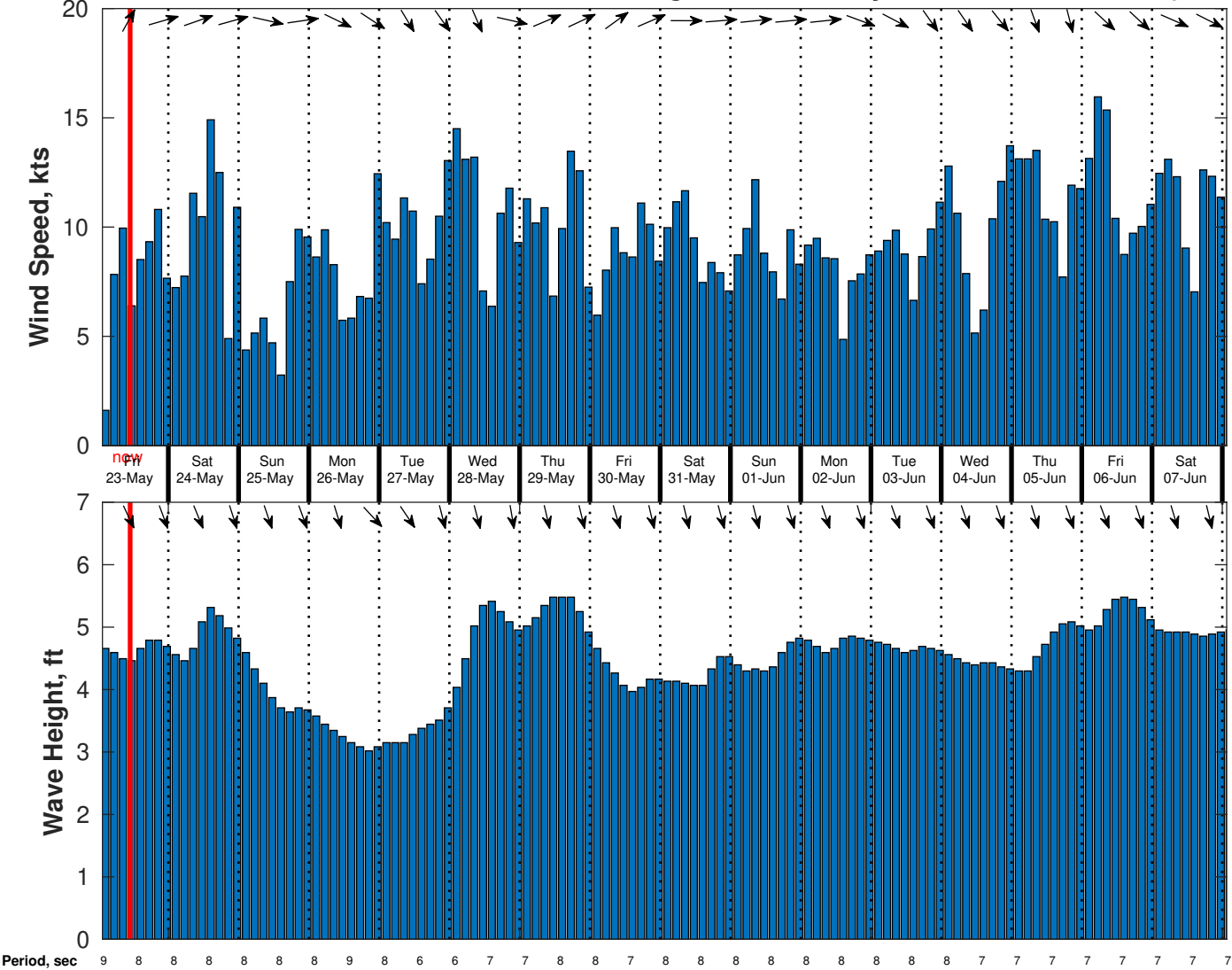
Wind & Wave Forecast for CSA (ONHYM) PPL EBS - Senegal from 22-May-2025 01:00:00 to 07-Jun-2025 01:00:00
