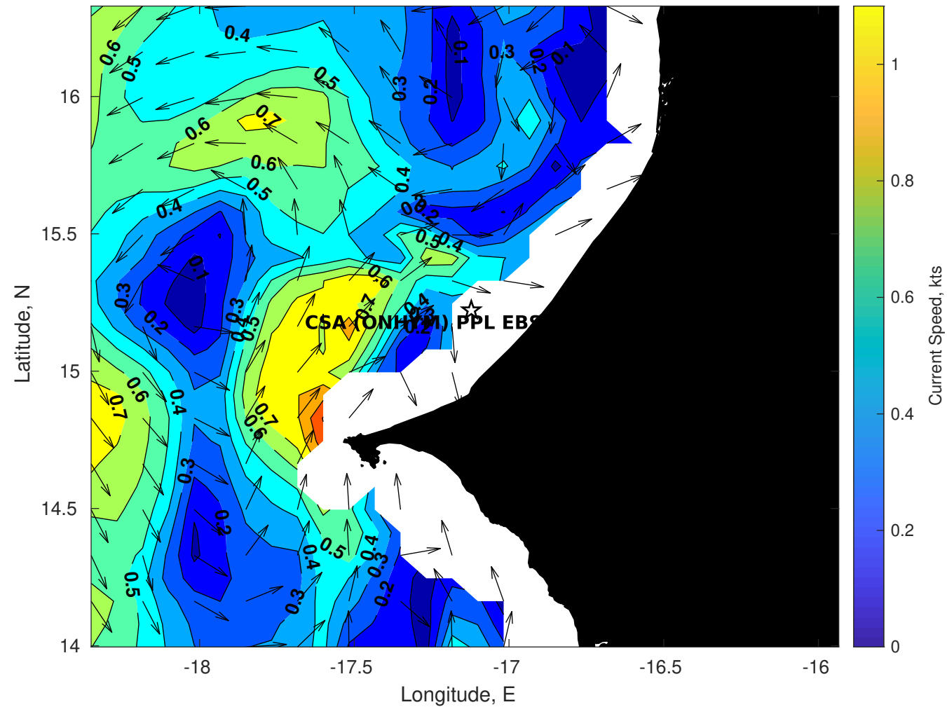
Surface Currents for CSA (ONHYM) PPL EBS - Senegal at 21-May-2025 00:00:00
