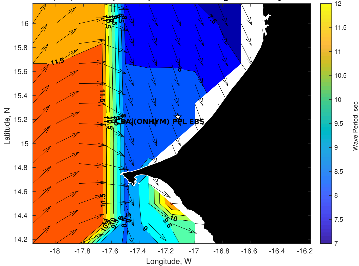
Wave Period (sec) for CSA (ONHYM) PPL EBS - Senegal at 22-May-2025 09:00:00
