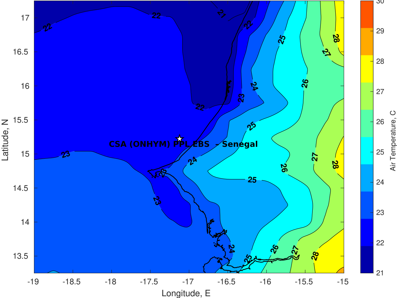
Air Temperature (C) for CSA (ONHYM) PPL EBS - Senegal at 22-May-2025
