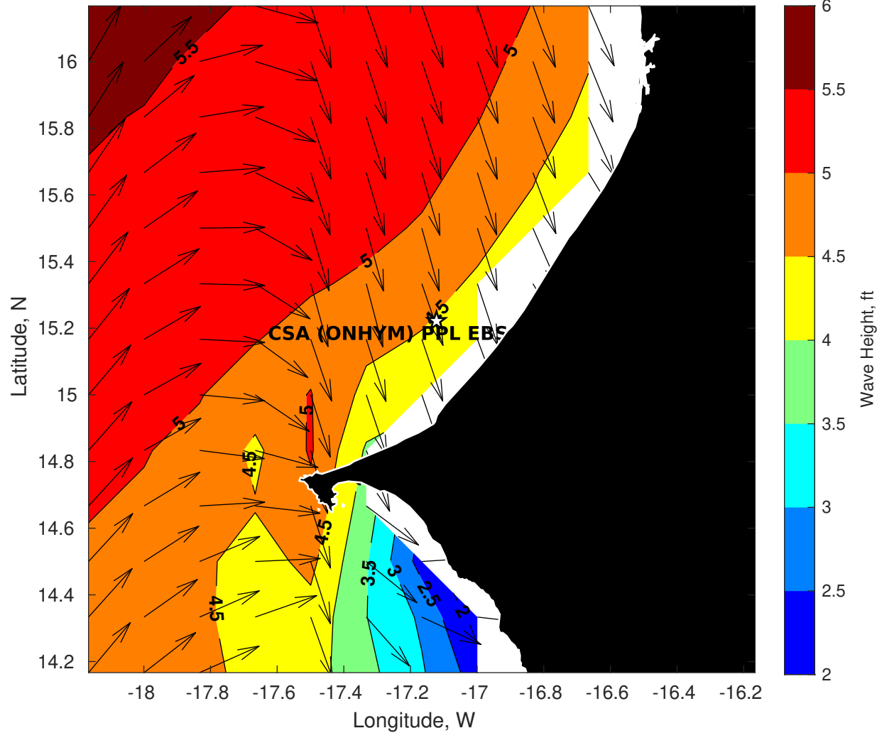
Wave Height (ft) for CSA (ONHYM) PPL EBS - Senegal at 22-May-2025 09:00:00
