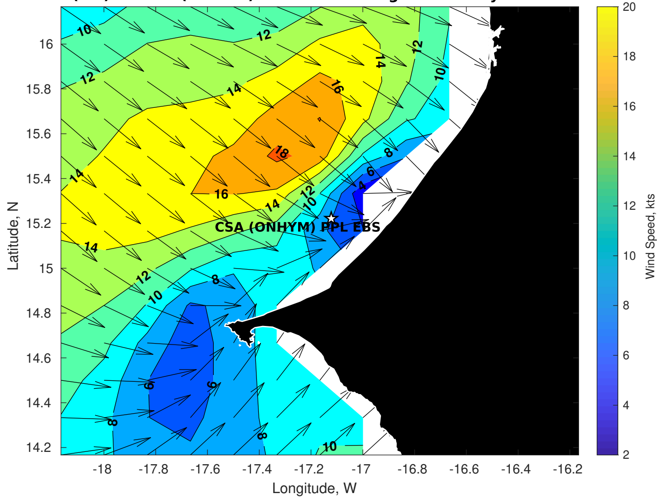
Winds (kts) for CSA (ONHYM) PPL EBS - Senegal at 22-May-2025 09:00:00
