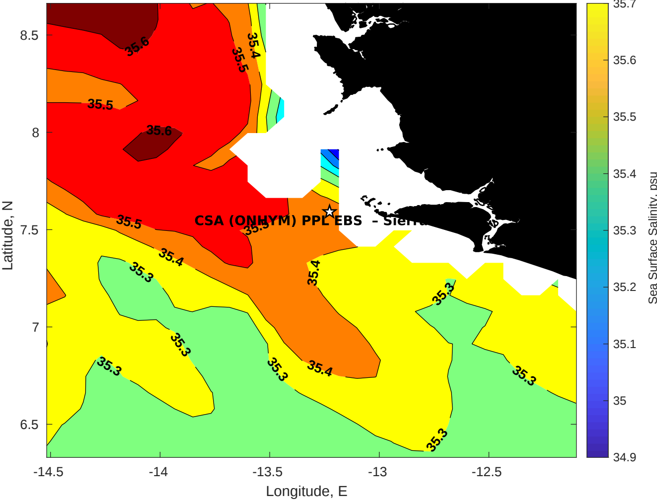
Surface Salinity for CSA (ONHYM) PPL EBS - Sierra Leone at 21-May-2025 00:00:00
