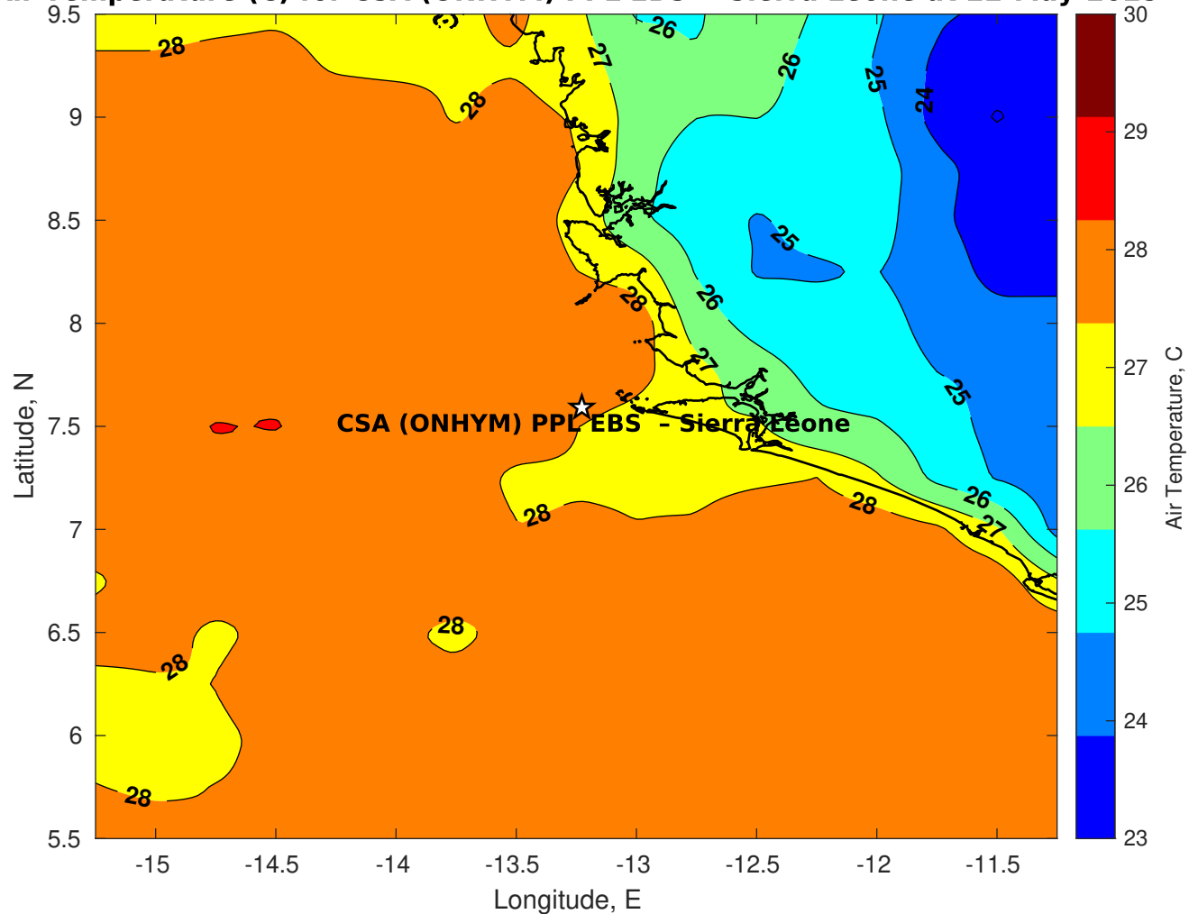
Air Temperature (C) for CSA (ONHYM) PPL EBS - Sierra Leone at 22-May-2025
