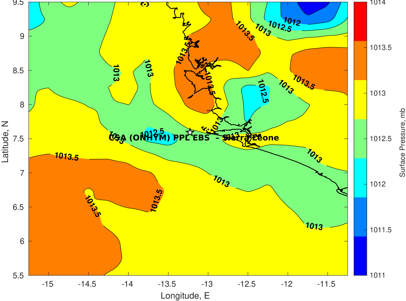
Surface Pressure (mb) for CSA (ONHYM) PPL EBS - Sierra Leone at 15-Nov-2030 00:00:00
