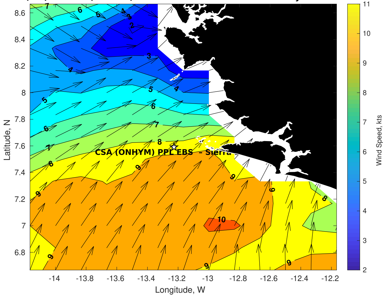
Winds (kts) for CSA (ONHYM) PPL EBS - Sierra Leone at 22-May-2025 09:00:00
