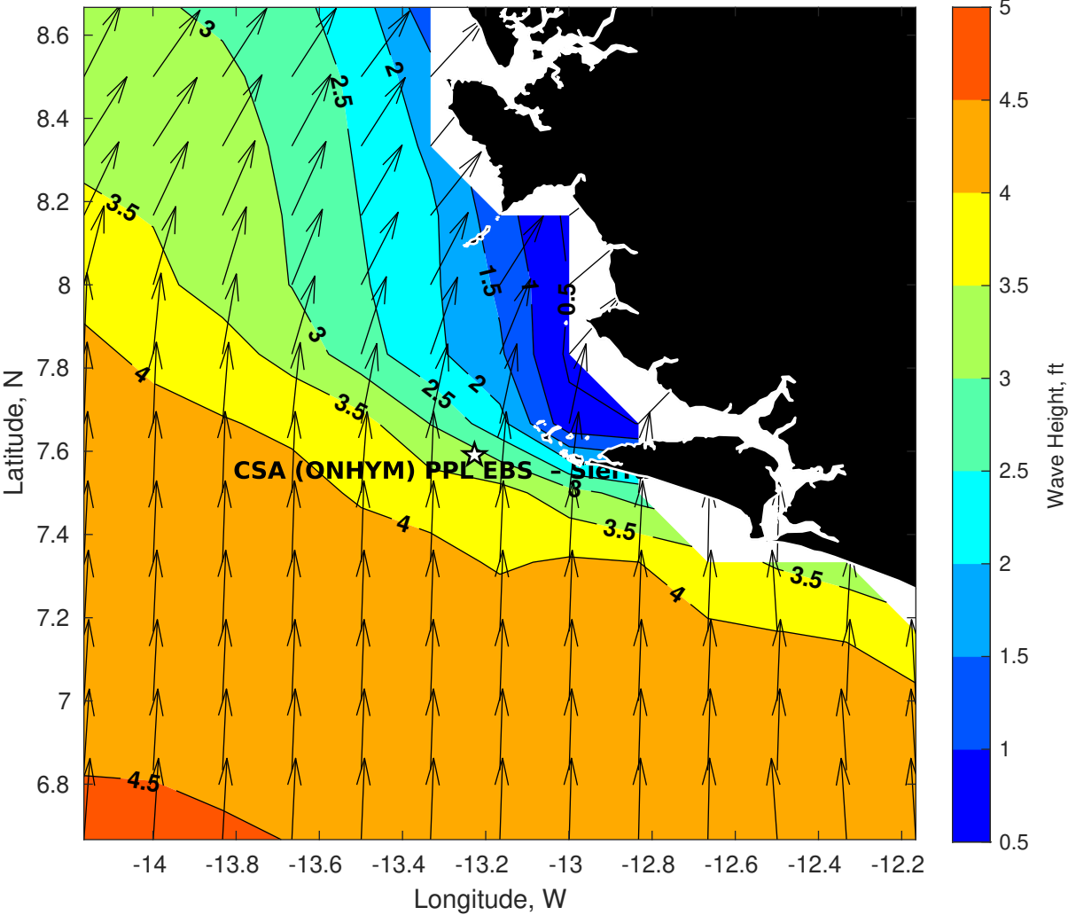
Wave Height (ft) for CSA (ONHYM) PPL EBS - Sierra Leone at 22-May-2025 09:00:00
