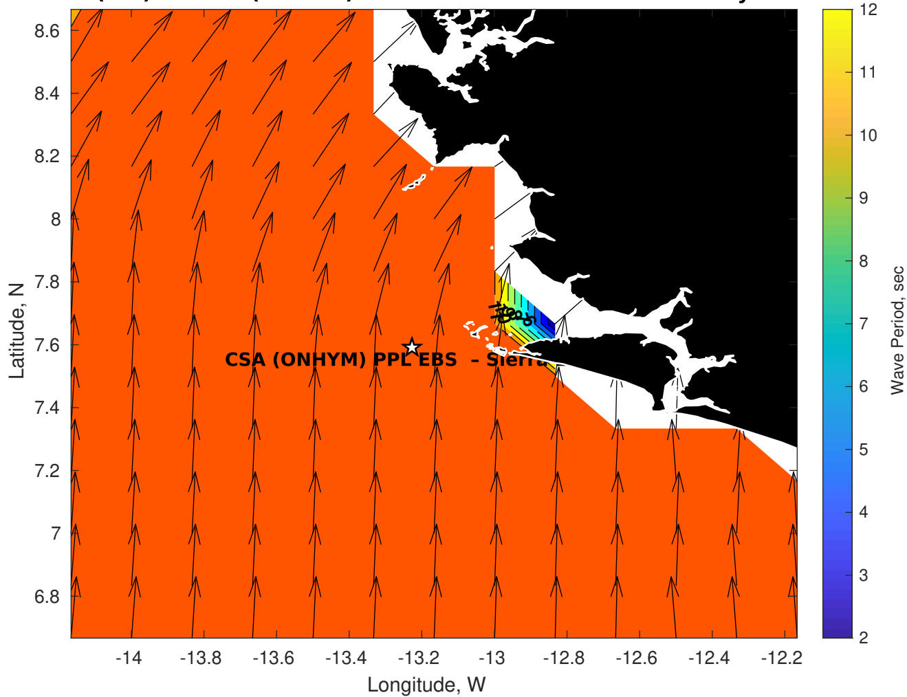
Wave Period (sec) for CSA (ONHYM) PPL EBS - Sierra Leone at 22-May-2025 09:00:00
