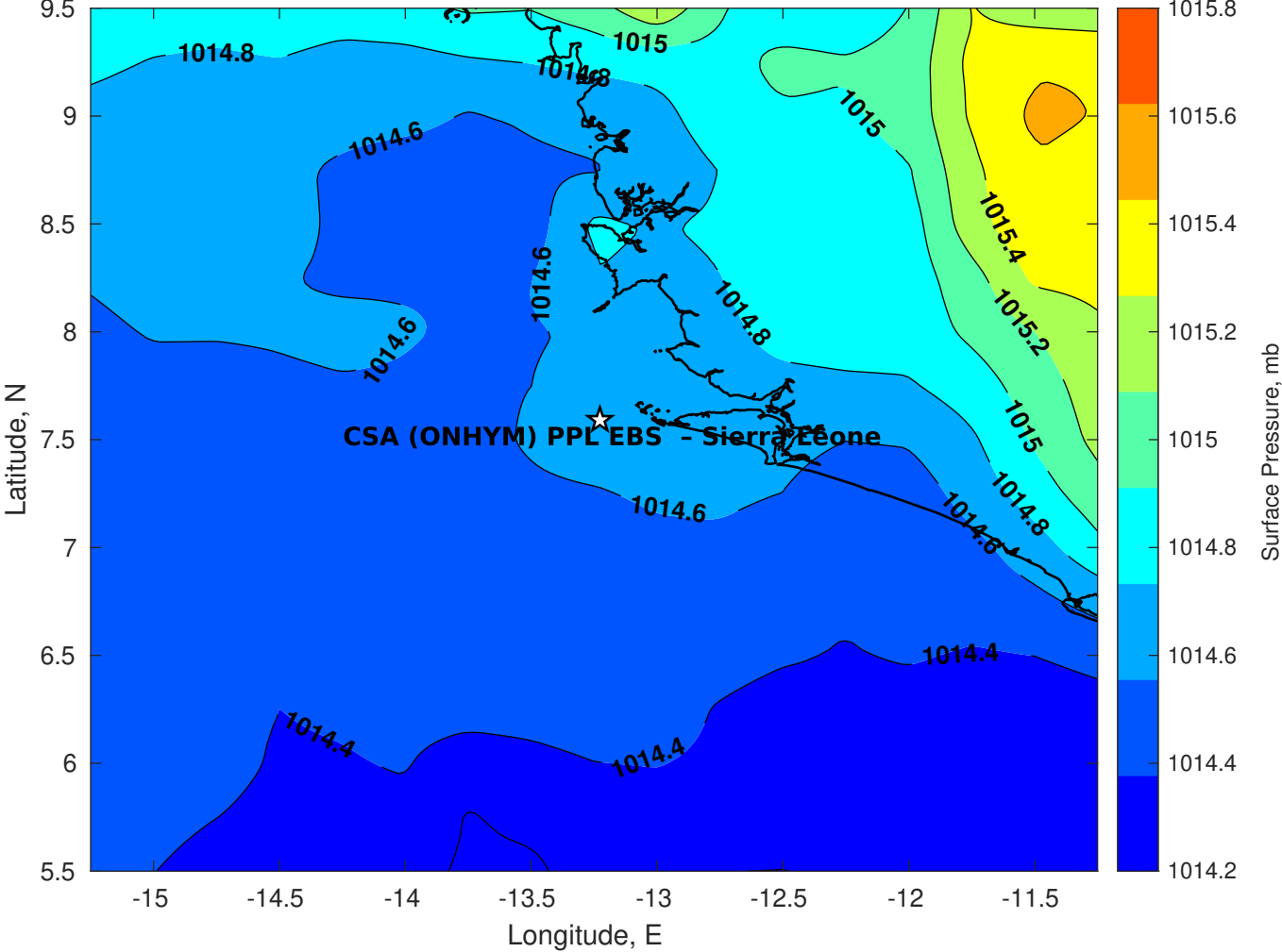
Surface Pressure (mb) for CSA (ONHYM) PPL EBS - Sierra Leone at 23-May-2025 00:00:00
