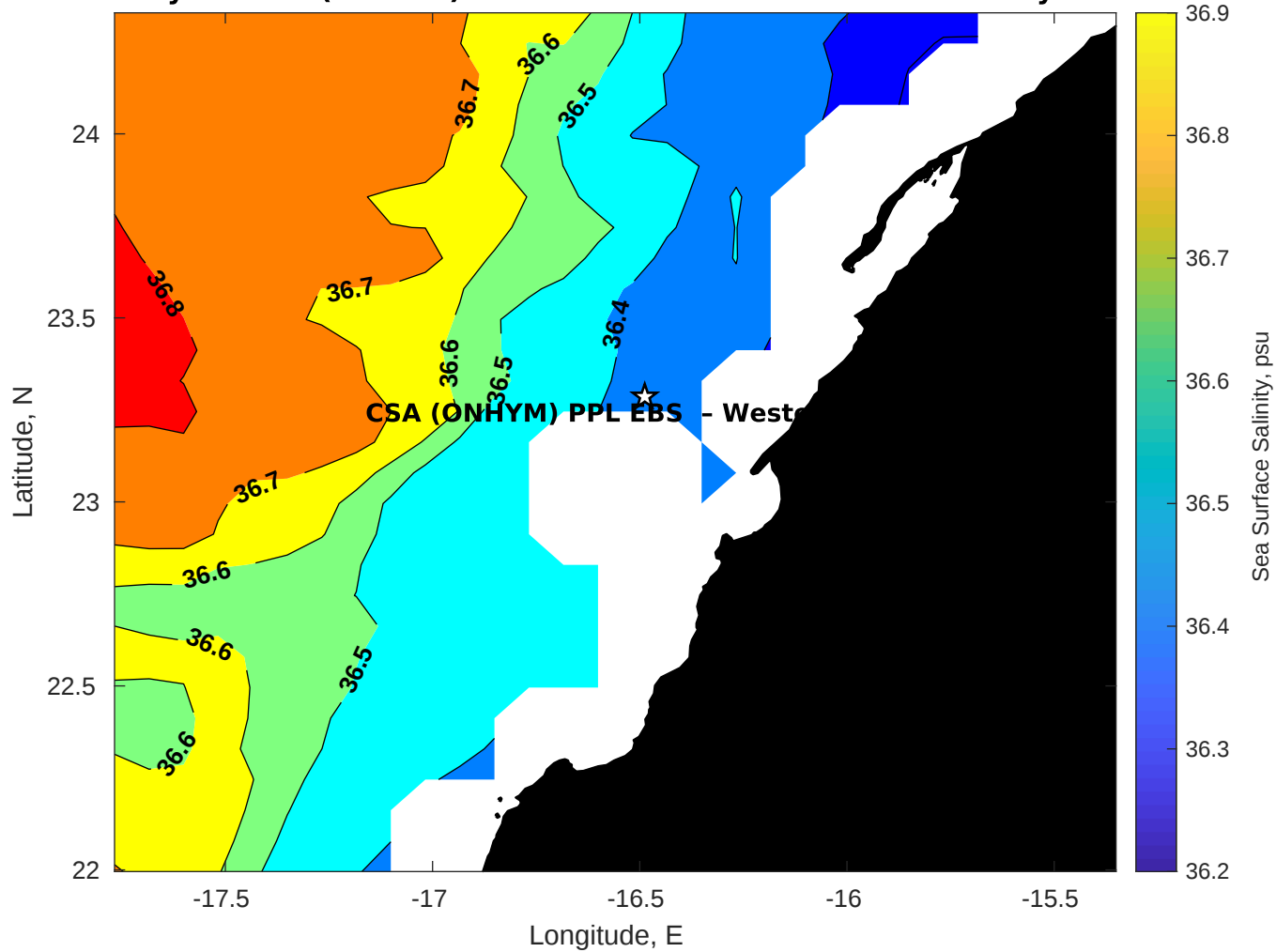
Surface Salinity for CSA (ONHYM) PPL EBS - Western Sahara at 21-May-2025 00:00:00
