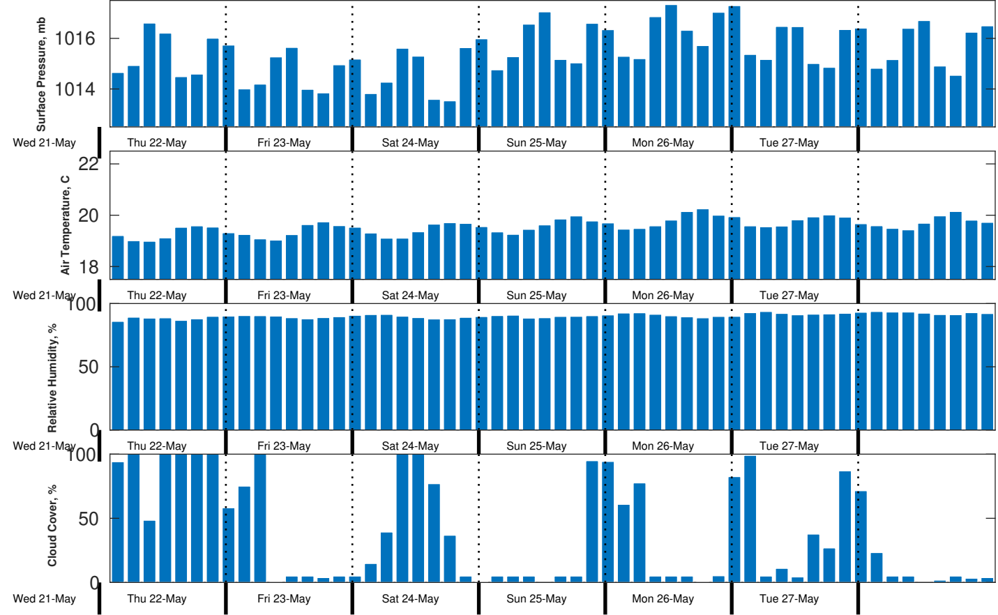
Met Forecast for CSA (ONHYM) PPL EBS - Western Sahara from 22-May-2025 00:00:00 to 29-May-2025 00:00:00
