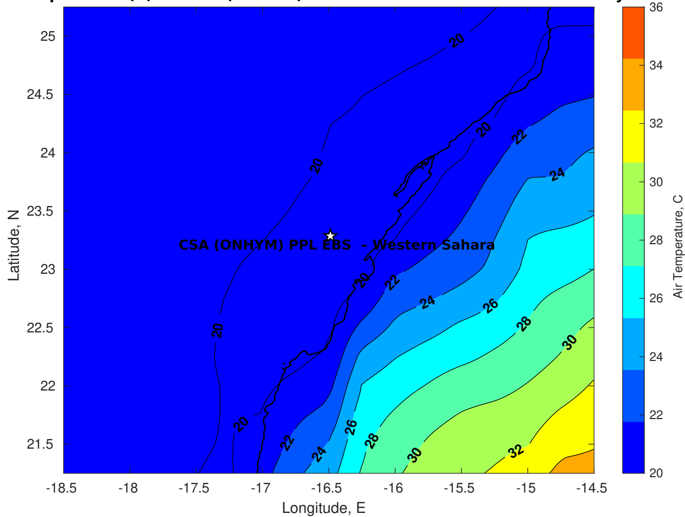
Air Temperature (C) for CSA (ONHYM) PPL EBS - Western Sahara at 22-May-2025
