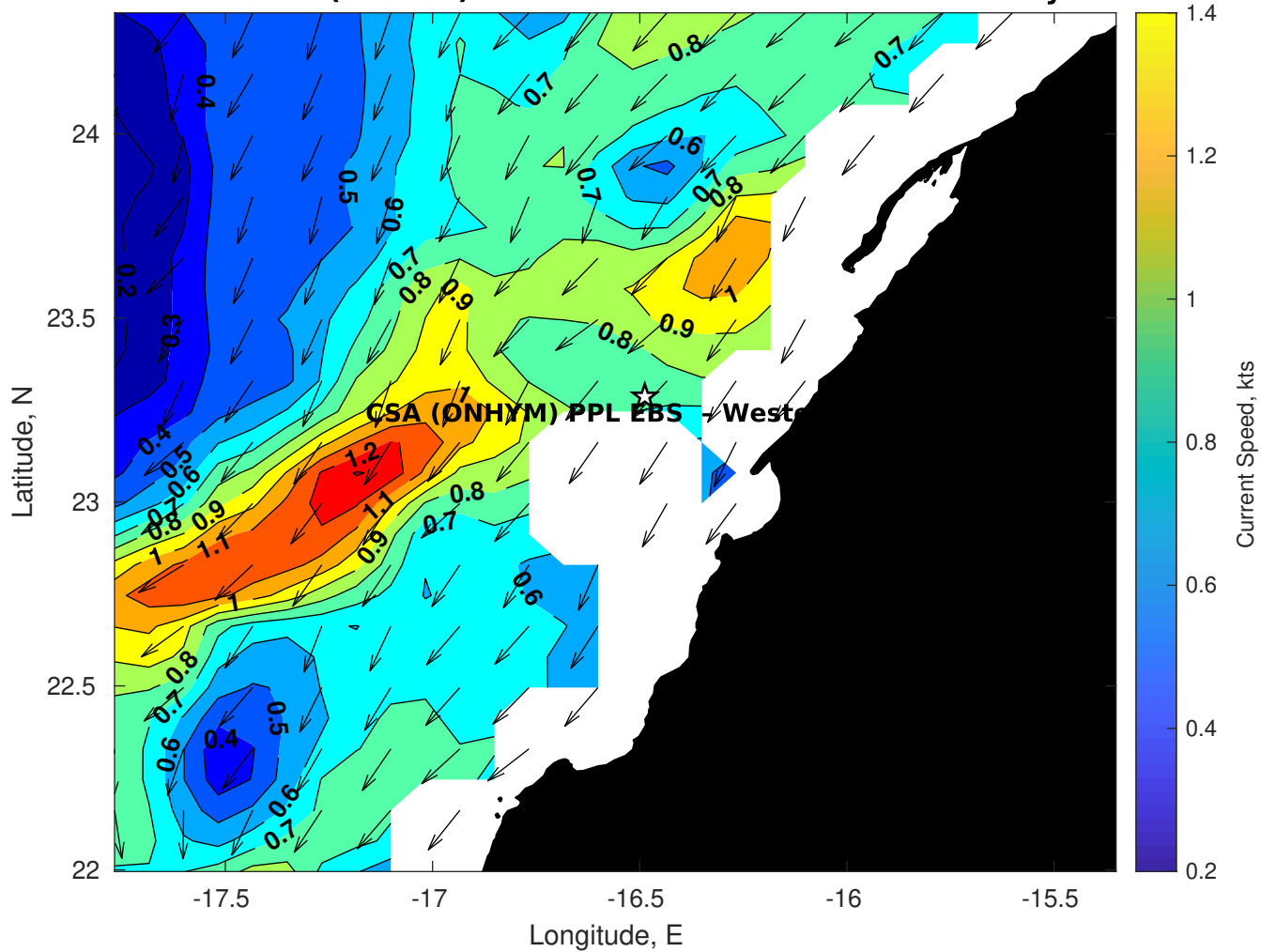
Surface Currents for CSA (ONHYM) PPL EBS - Western Sahara at 21-May-2025 00:00:00
