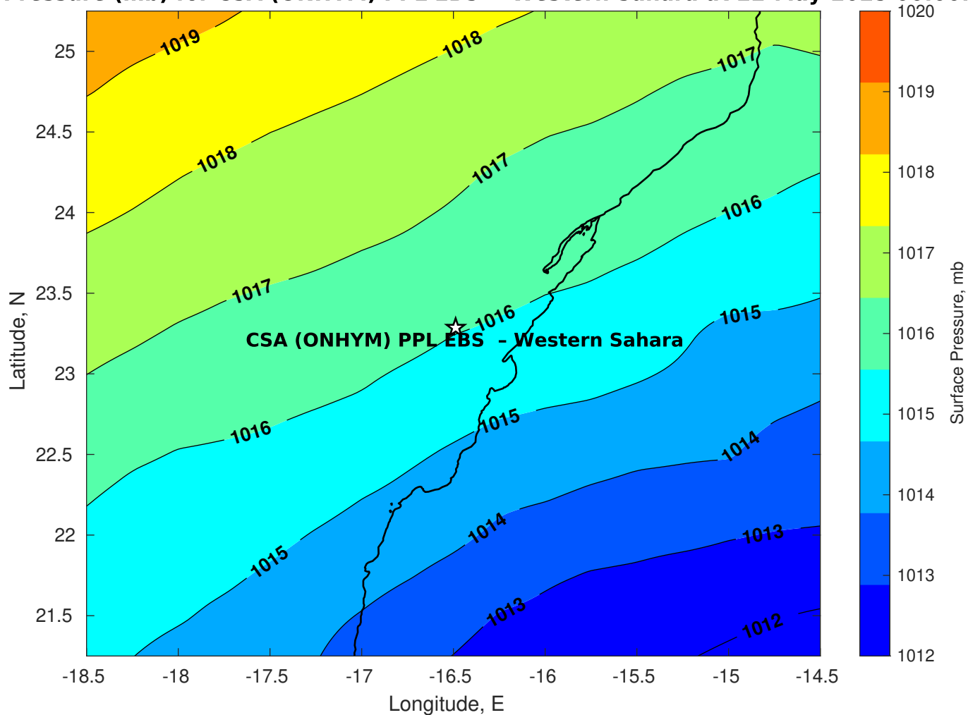
Surface Pressure (mb) for CSA (ONHYM) PPL EBS - Western Sahara at 22-May-2025 00:00:00
