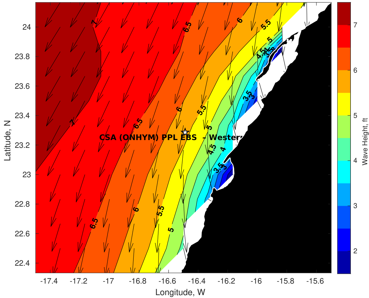
Wave Height (ft) for CSA (ONHYM) PPL EBS - Western Sahara at 22-May-2025 09:00:00
