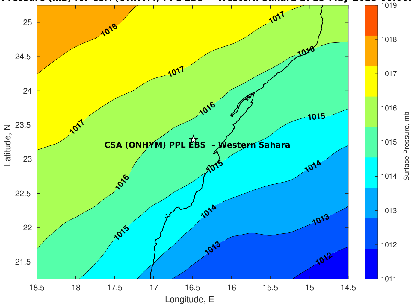
Surface Pressure (mb) for CSA (ONHYM) PPL EBS - Western Sahara at 23-May-2025 00:00:00
