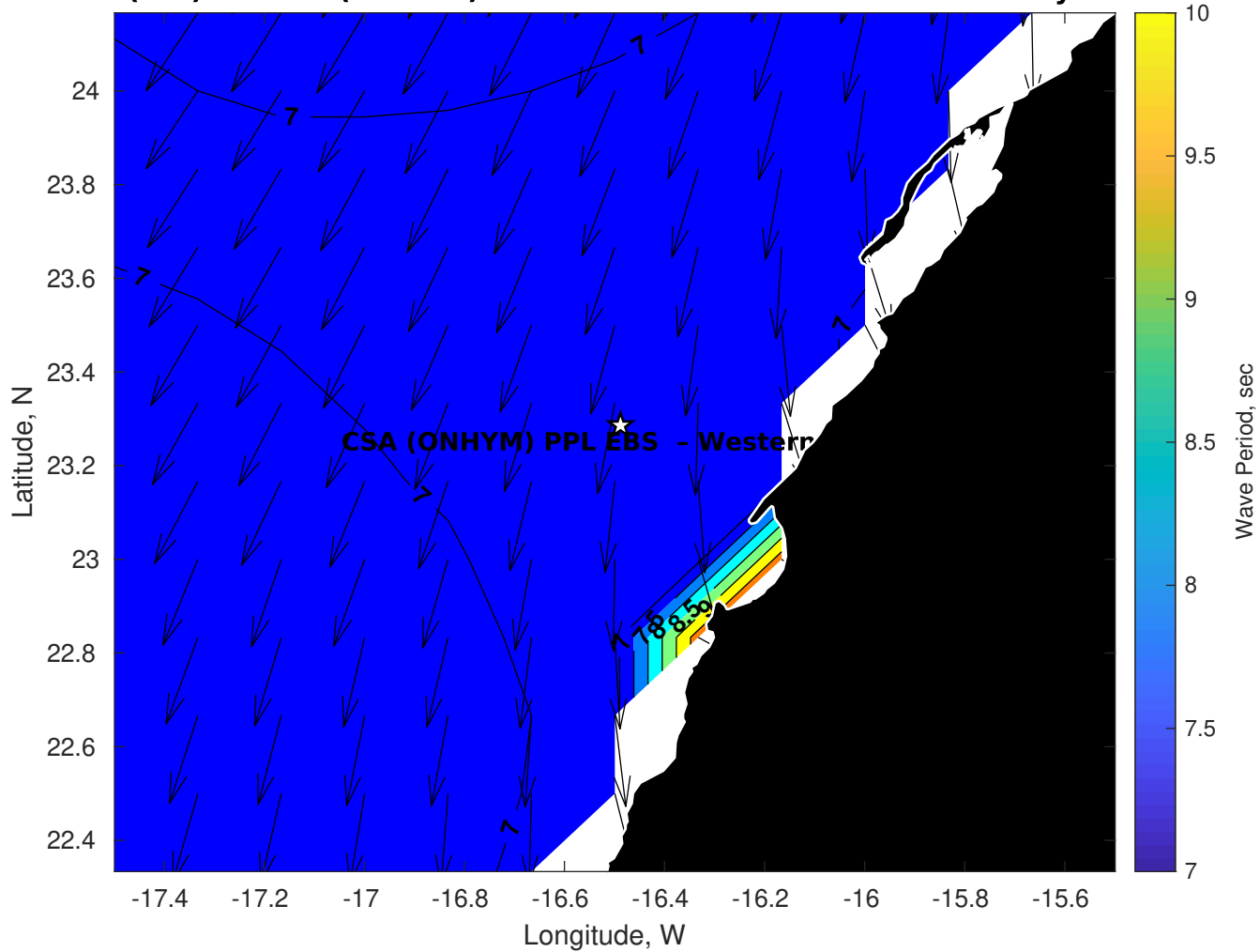
Wave Period (sec) for CSA (ONHYM) PPL EBS - Western Sahara at 22-May-2025 09:00:00
