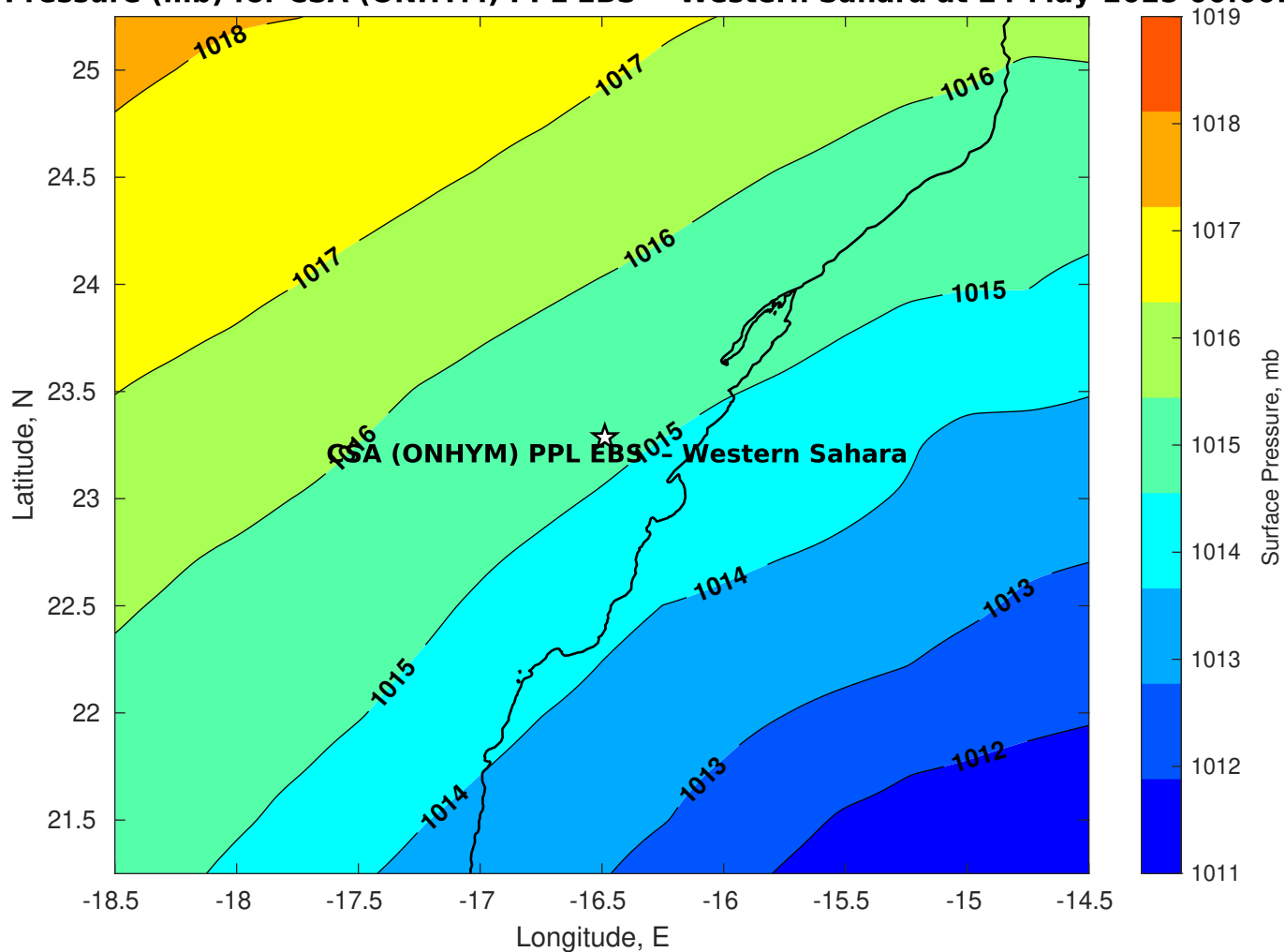
Surface Pressure (mb) for CSA (ONHYM) PPL EBS - Western Sahara at 24-May-2025 00:00:00
