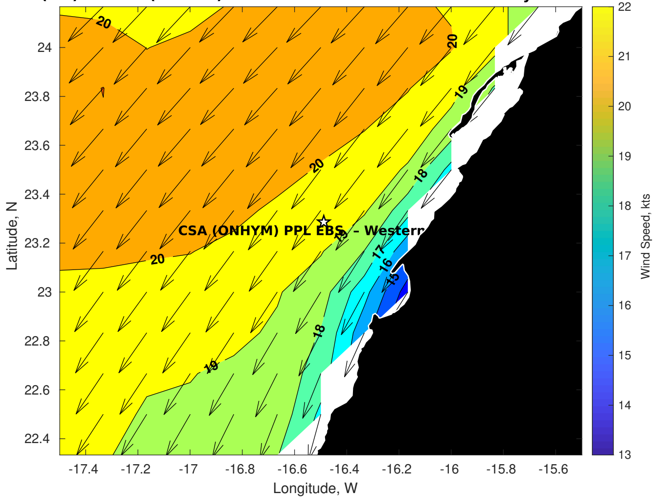
Winds (kts) for CSA (ONHYM) PPL EBS - Western Sahara at 22-May-2025 09:00:00
