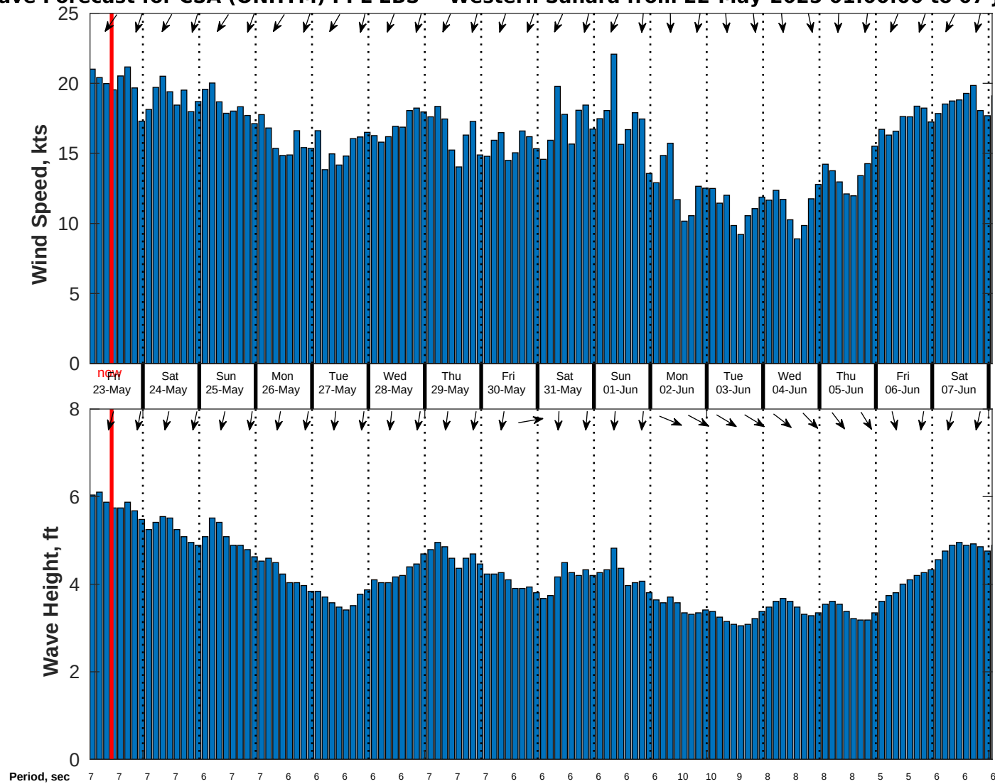
Wind & Wave Forecast for CSA (ONHYM) PPL EBS - Western Sahara from 22-May-2025 01:00:00 to 07-Jun-2025 01:00:00
