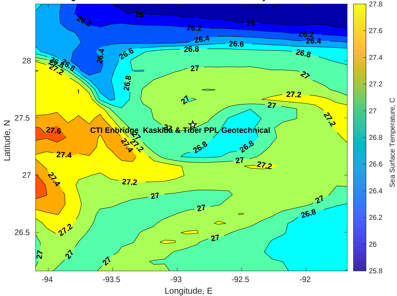
SST for CTI Enbridge Kaskida & Tiber PPL Geotechnical at 21-May-2025 00:00:00
