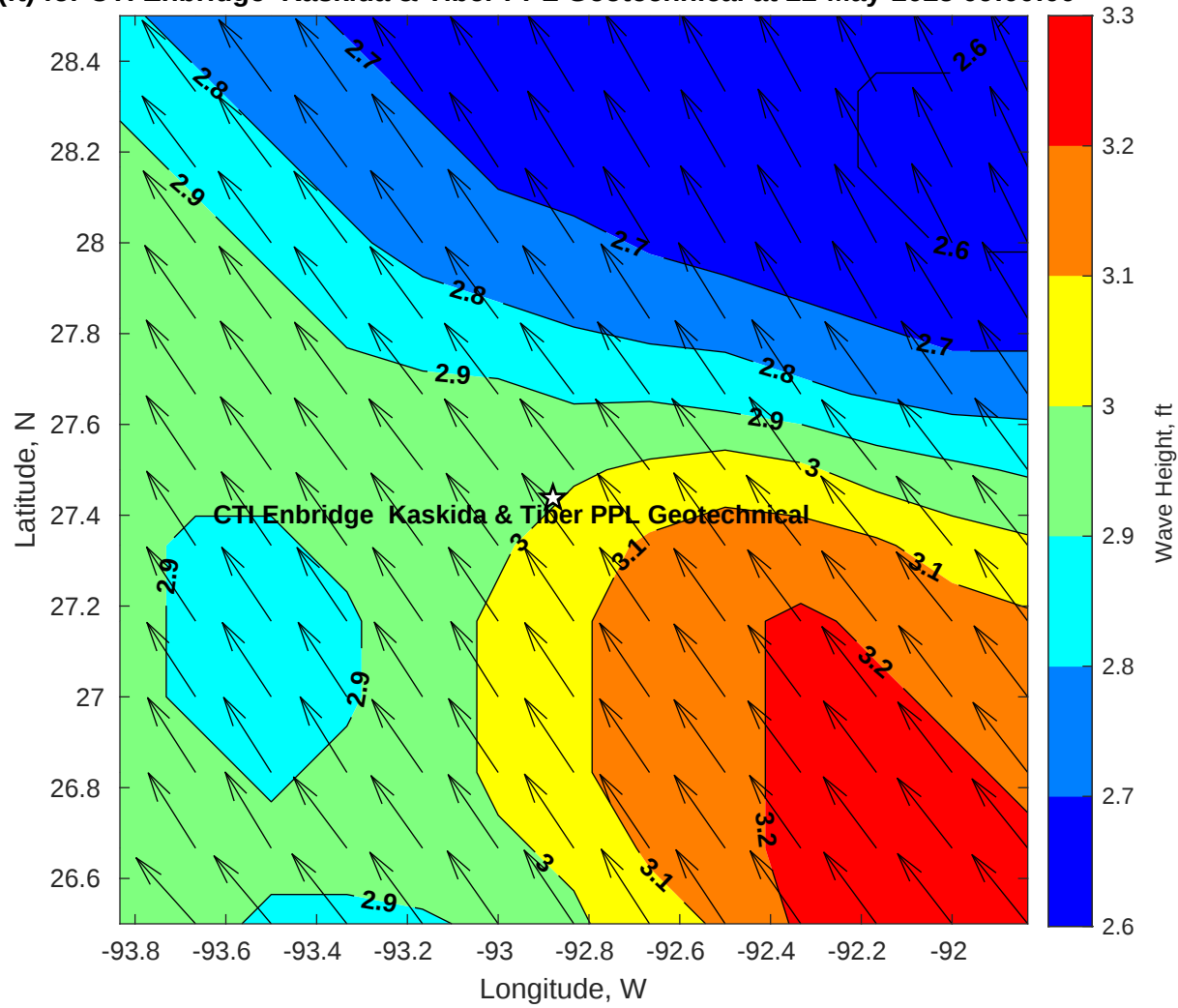
Wave Height (ft) for CTI Enbridge Kaskida & Tiber PPL Geotechnical at 22-May-2025 09:00:00
