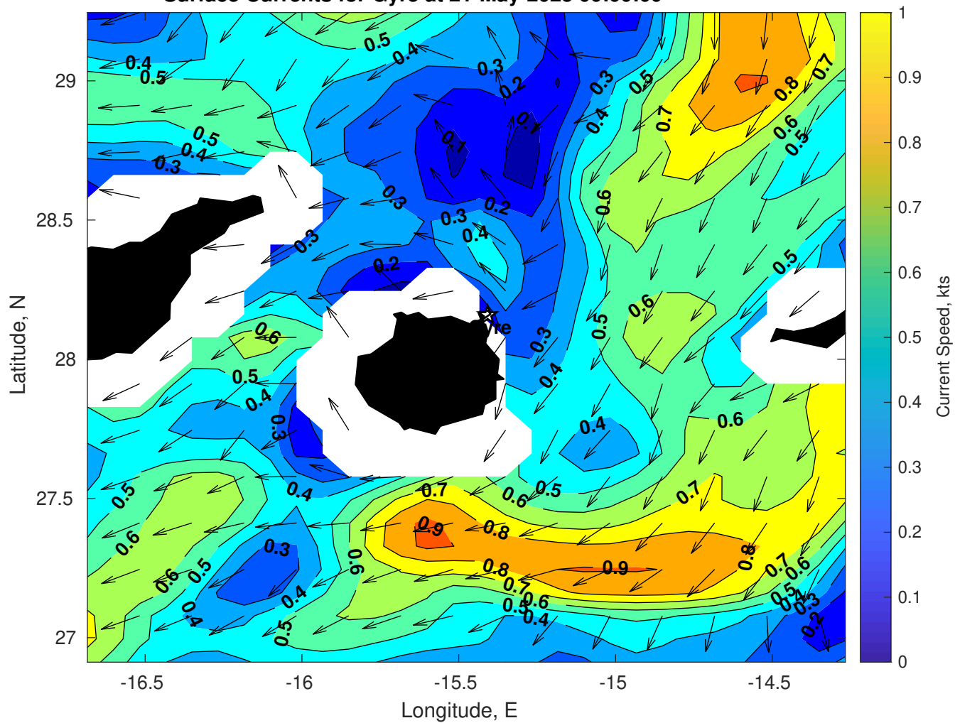
Surface Currents for Gyre at 21-May-2025 00:00:00
