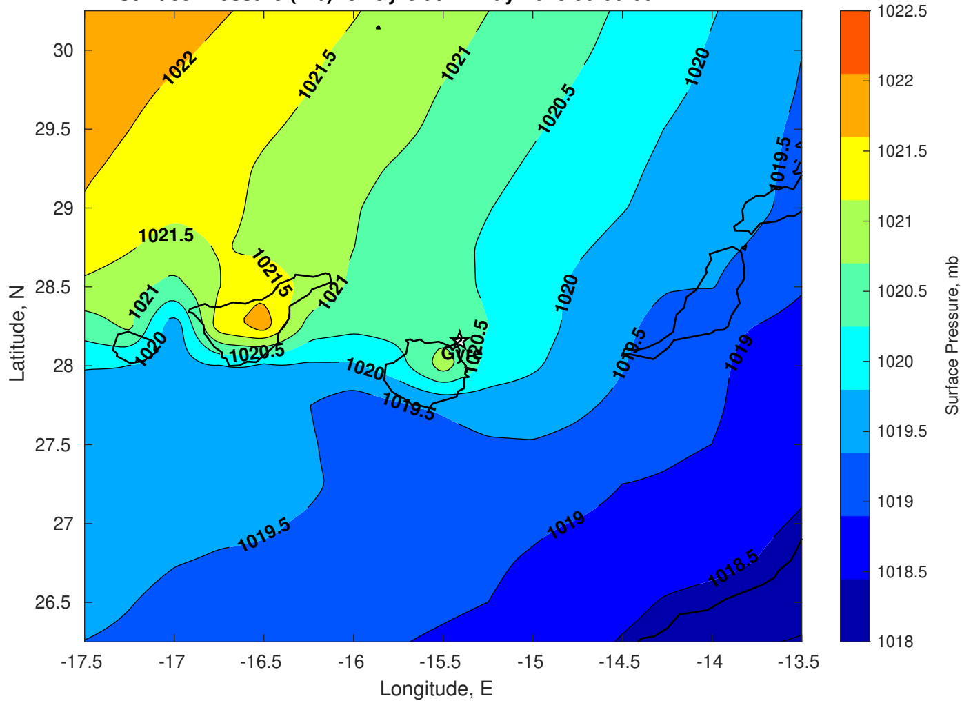
Surface Pressure (mb) for Gyre at 22-May-2025 00:00:00
