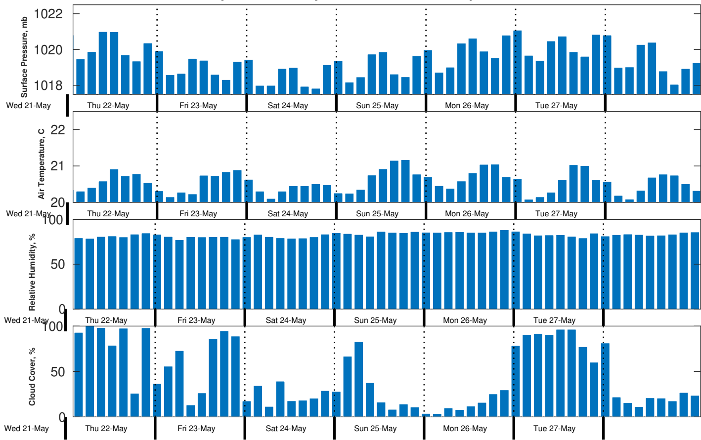
Met Forecast for Gyre from 21-May-2025 23:00:00 to 28-May-2025 23:00:00
