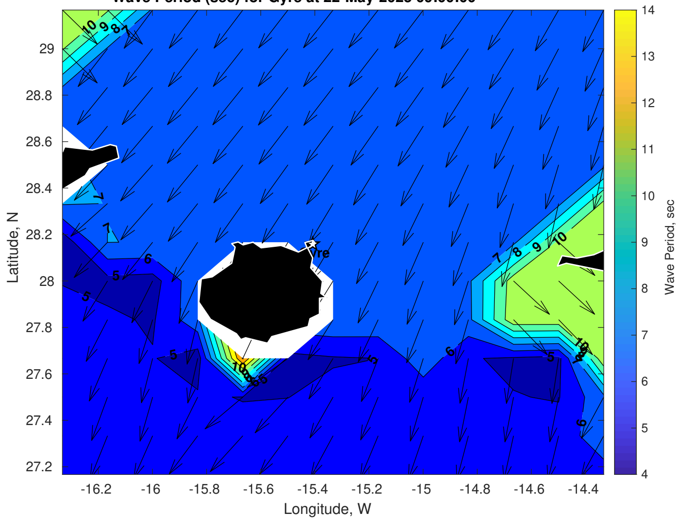
Wave Period (sec) for Gyre at 22-May-2025 09:00:00
