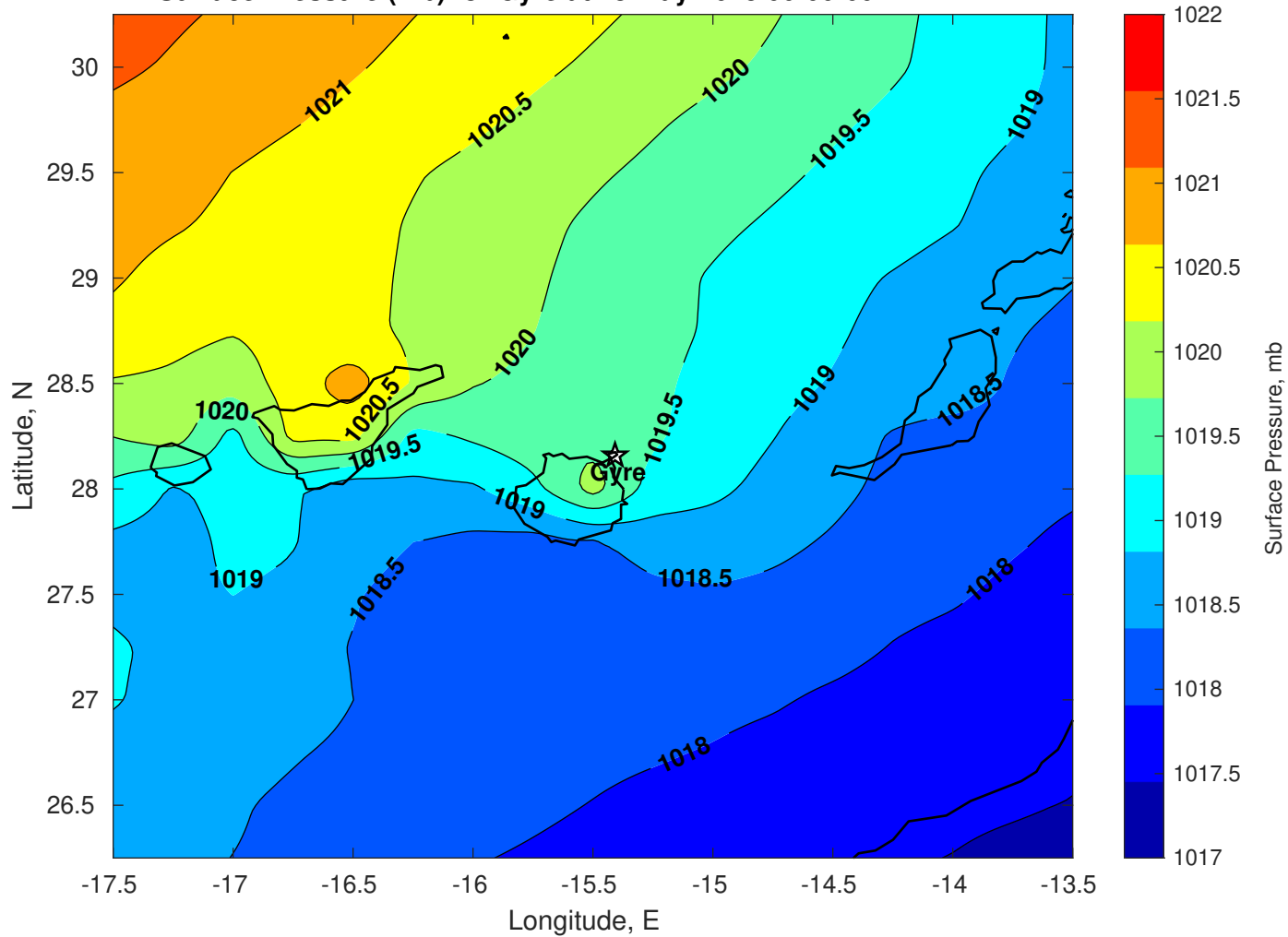
Surface Pressure (mb) for Gyre at 23-May-2025 00:00:00
