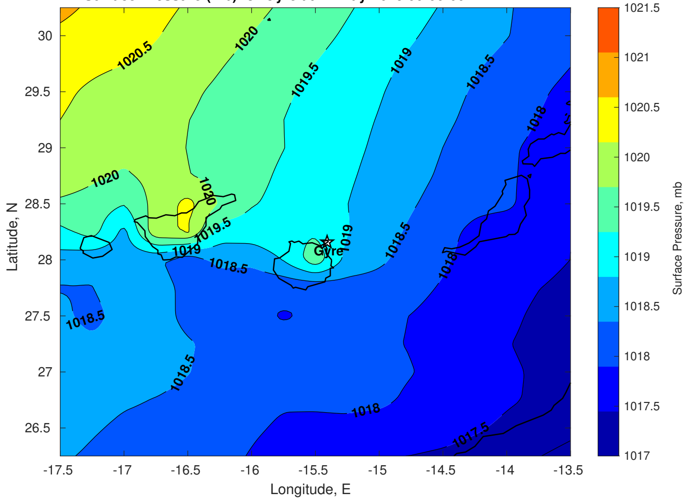
Surface Pressure (mb) for Gyre at 24-May-2025 00:00:00
