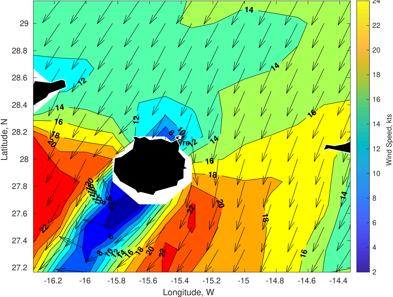
Winds (kts) for Gyre at 22-May-2025 09:00:00
