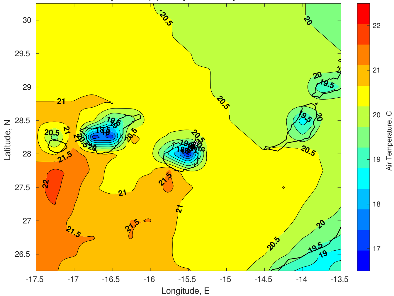
Air Temperature (C) for Gyre at 22-May-2025
