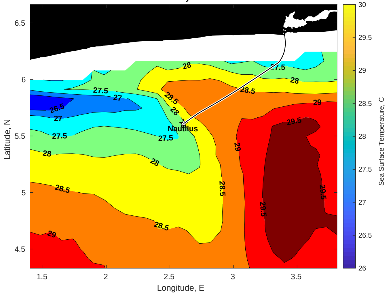
SST for Nautilus at 21-May-2025 00:00:00
