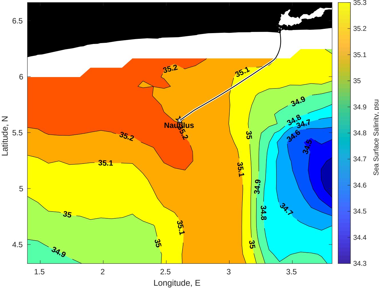
Surface Salinity for Nautilus at 21-May-2025 00:00:00
