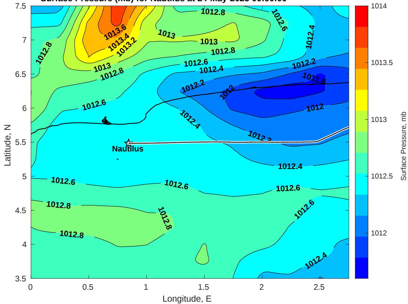
Surface Pressure (mb) for Nautilus at 24-May-2025 00:00:00
