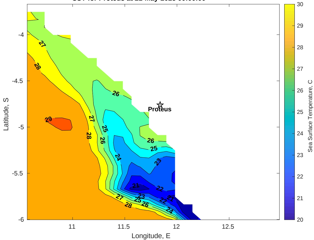
SST for Proteus at 21-May-2025 00:00:00
