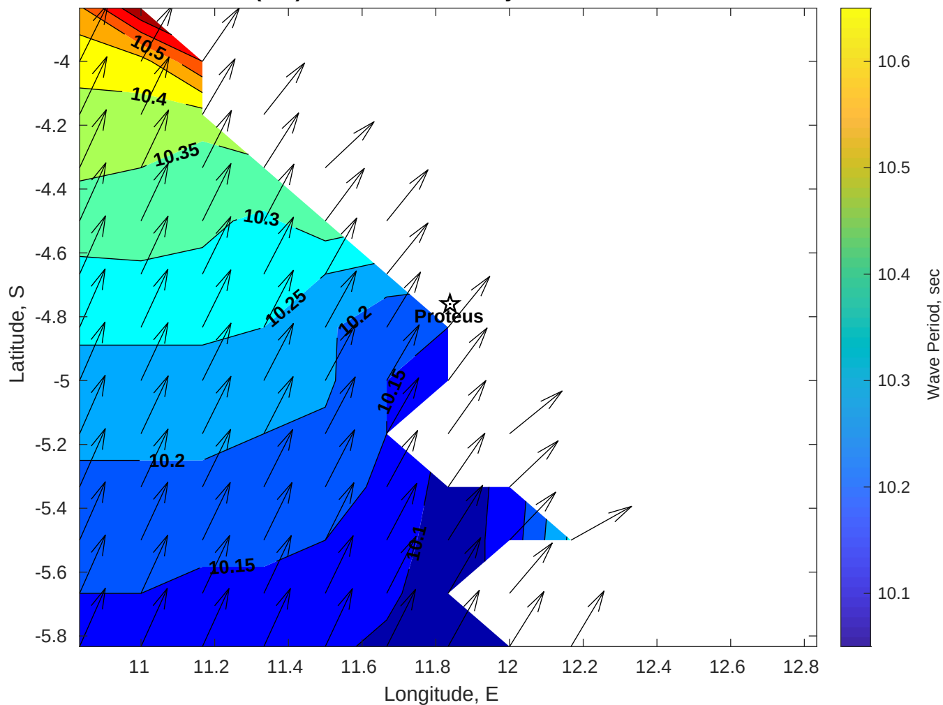
Wave Period (sec) for Proteus at 22-May-2025 09:00:00
