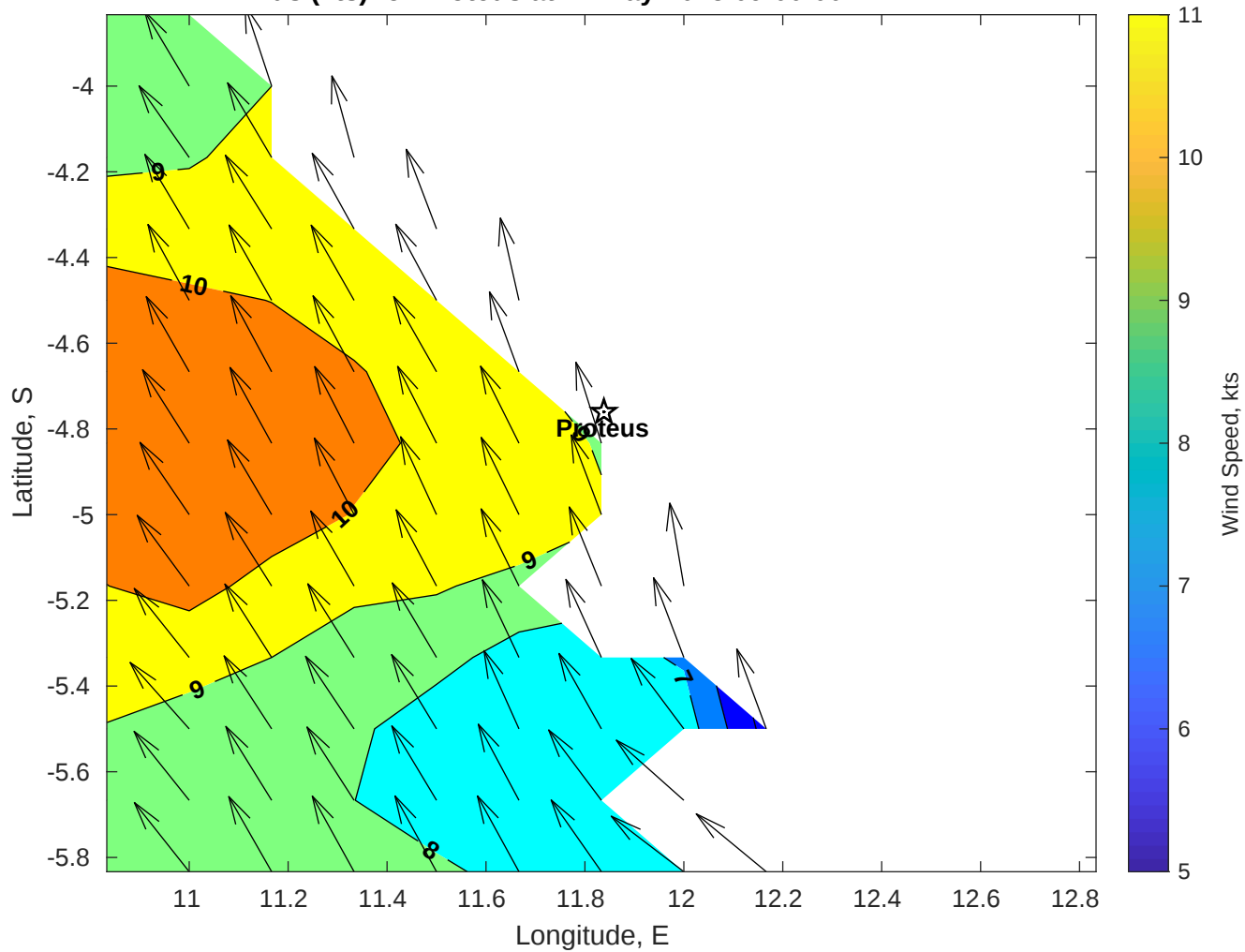
Winds (kts) for Proteus at 22-May-2025 09:00:00
