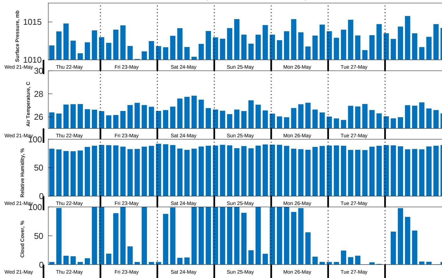
Met Forecast for Proteus from 22-May-2025 00:00:00 to 29-May-2025 00:00:00
