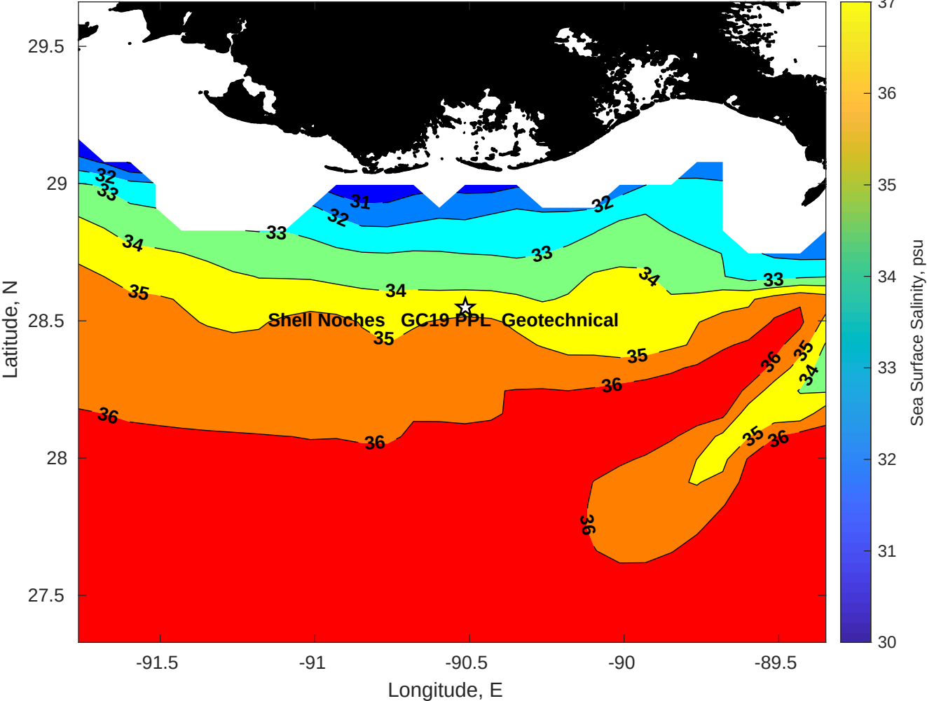
Surface Salinity for Shell Noches GC19 PPL Geotechnical at 21-May-2025 00:00:00
