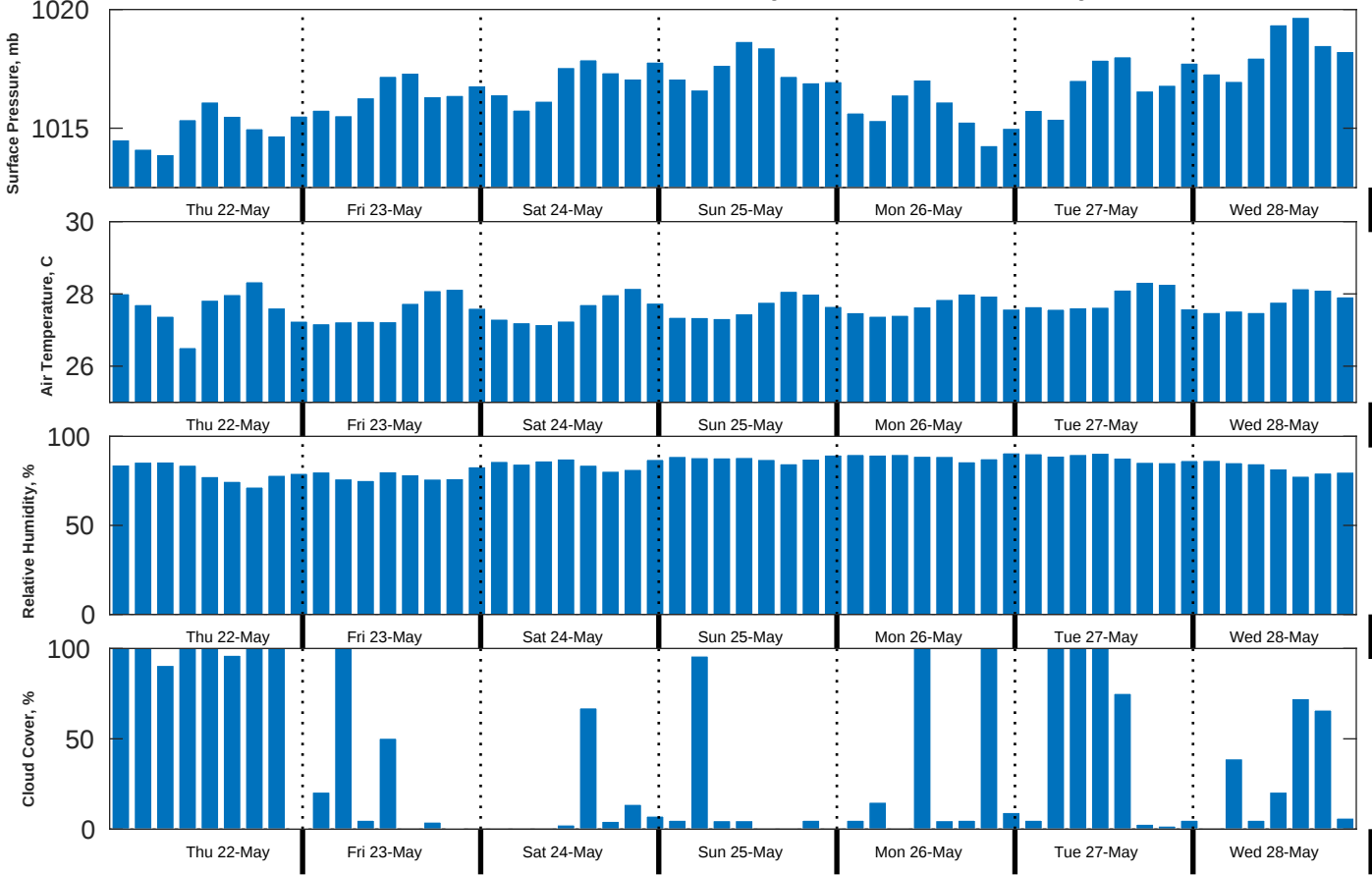
Met Forecast for Shell Noches GC19 PPL Geotechnical from 22-May-2025 00:00:00 to 29-May-2025 00:00:00
