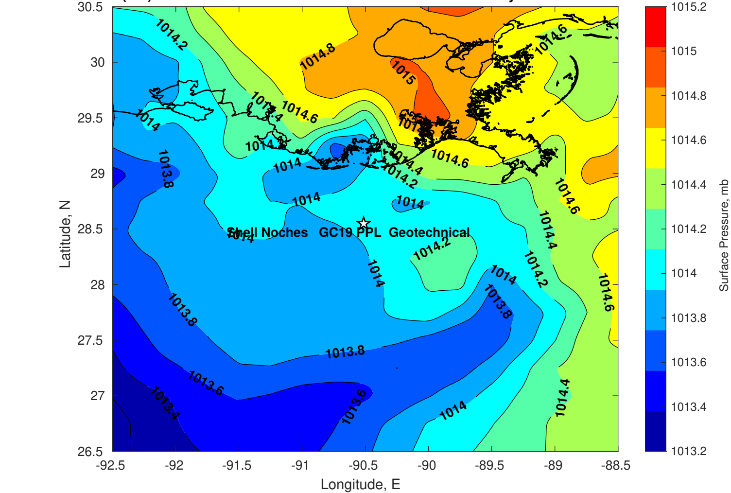
Surface Pressure (mb) for Shell Noches GC19 PPL Geotechnical at 22-May-2025 00:00:00
