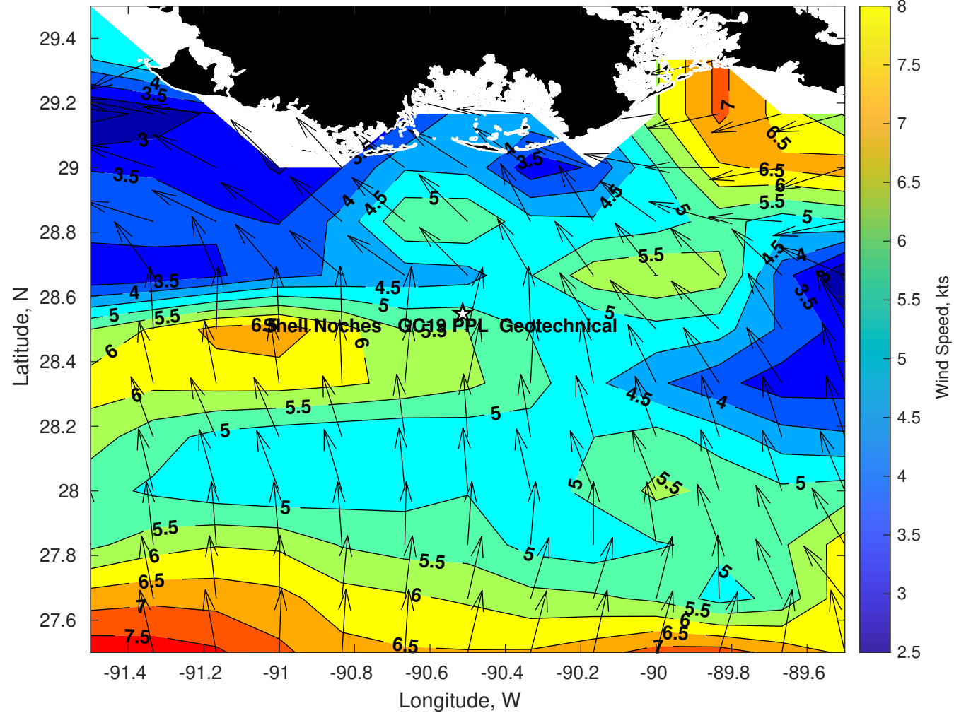
Winds (kts) for Shell Noches GC19 PPL Geotechnical at 22-May-2025 09:00:00
