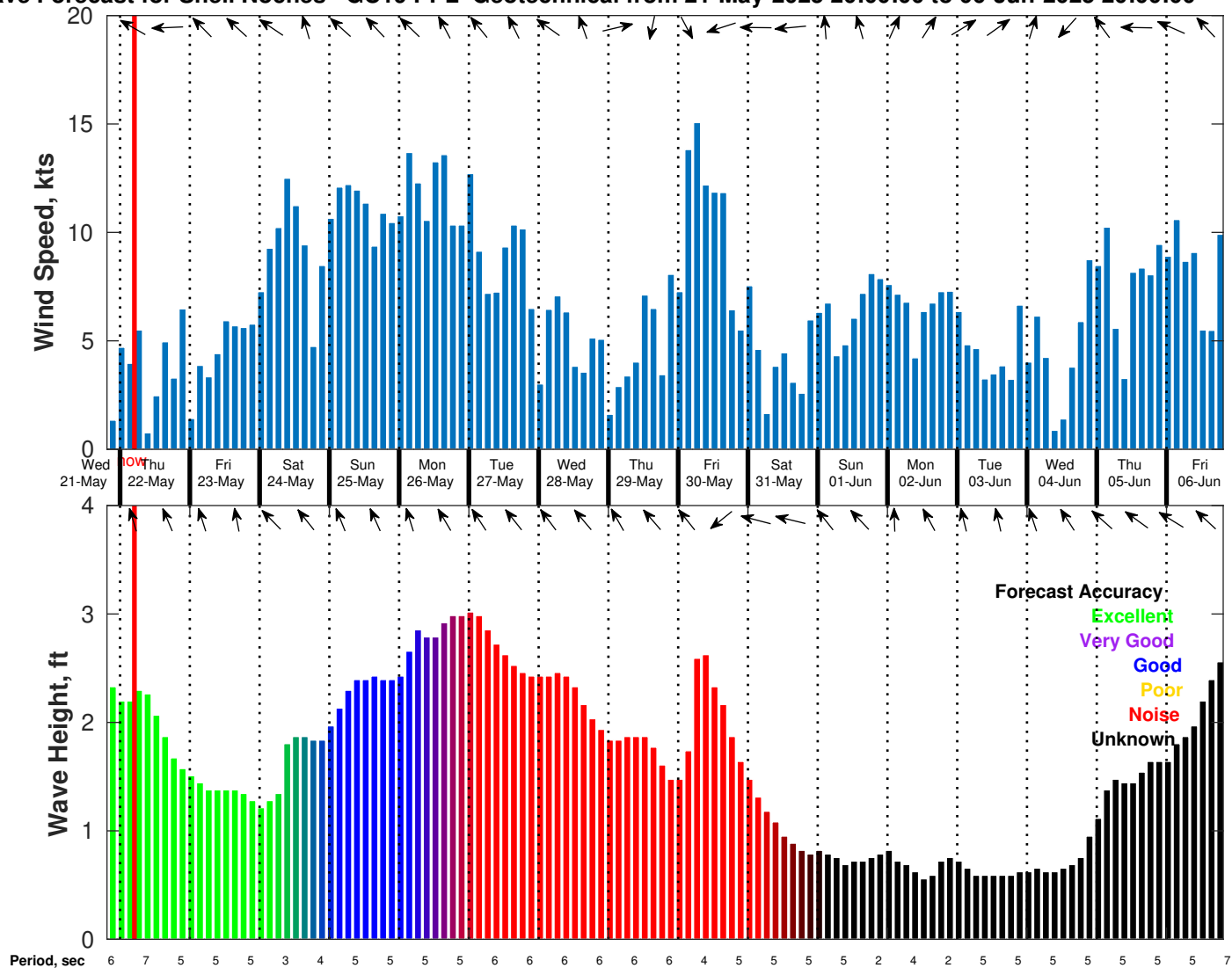
Wind & Wave Forecast for Shell Noches GC19 PPL Geotechnical from 21-May-2025 20:00:00 to 06-Jun-2025 20:00:00
