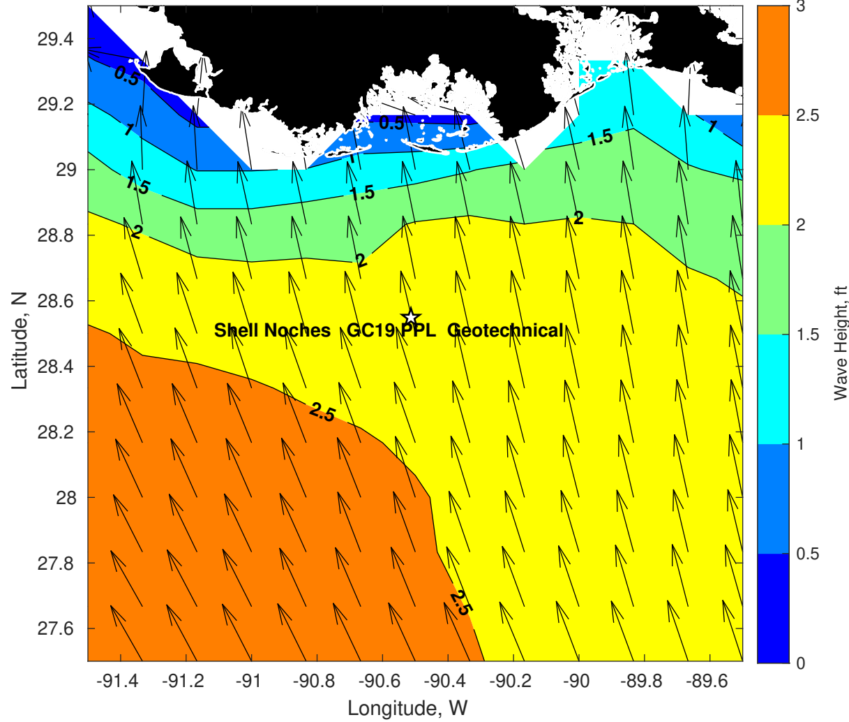
Wave Height (ft) for Shell Noches GC19 PPL Geotechnical at 22-May-2025 09:00:00
