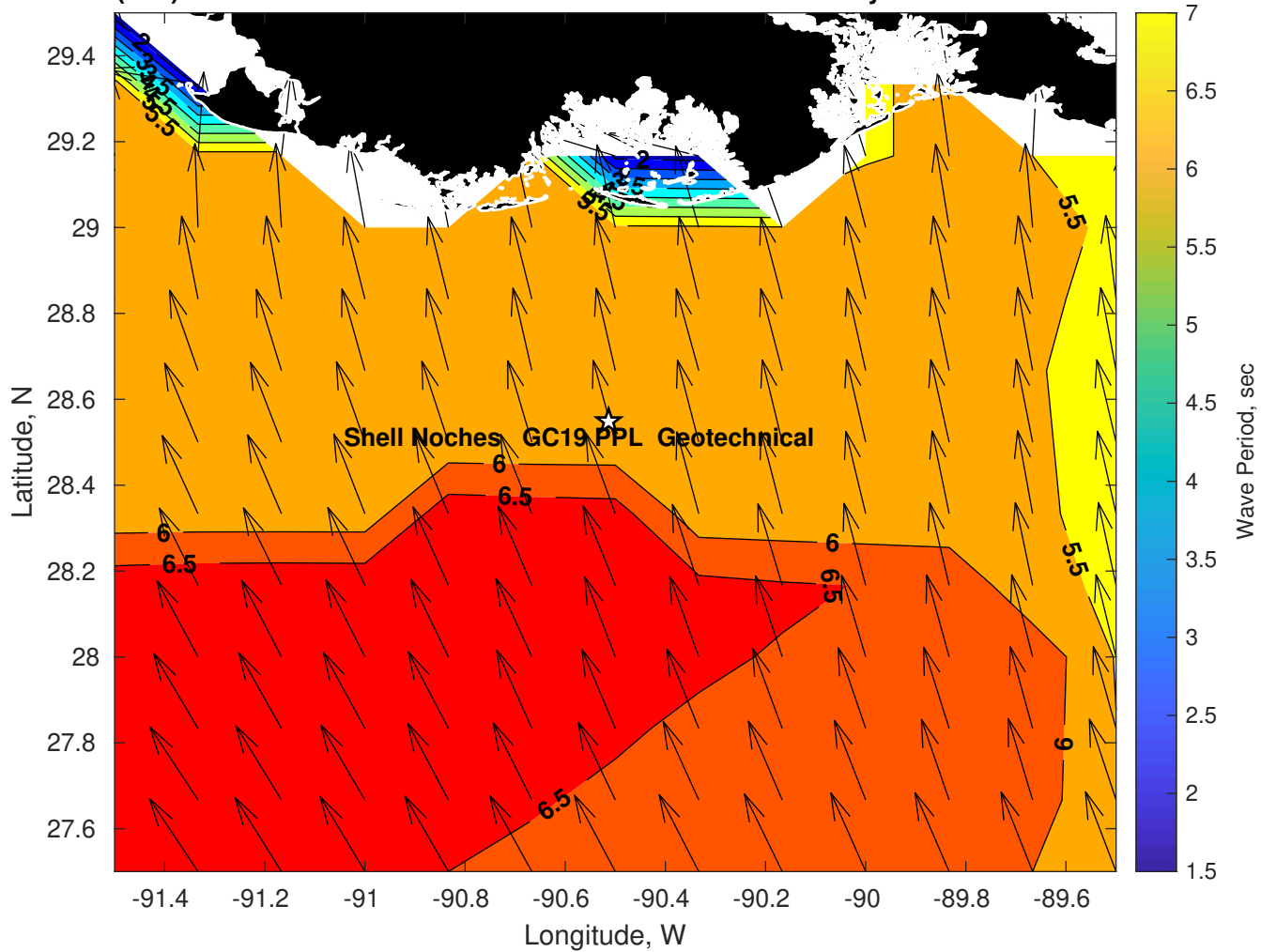
Wave Period (sec) for Shell Noches GC19 PPL Geotechnical at 22-May-2025 09:00:00
