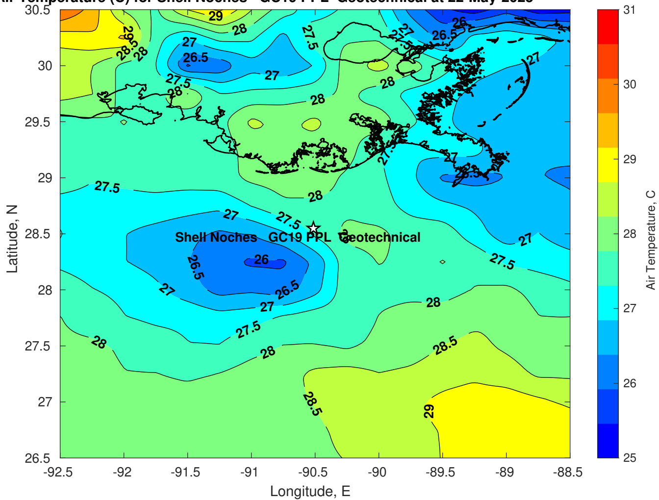
Air Temperature (C) for Shell Noches GC19 PPL Geotechnical at 22-May-2025
