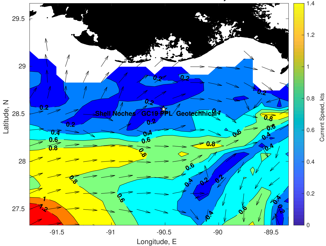
Surface Currents for Shell Noches GC19 PPL Geotechnical at 21-May-2025 00:00:00
