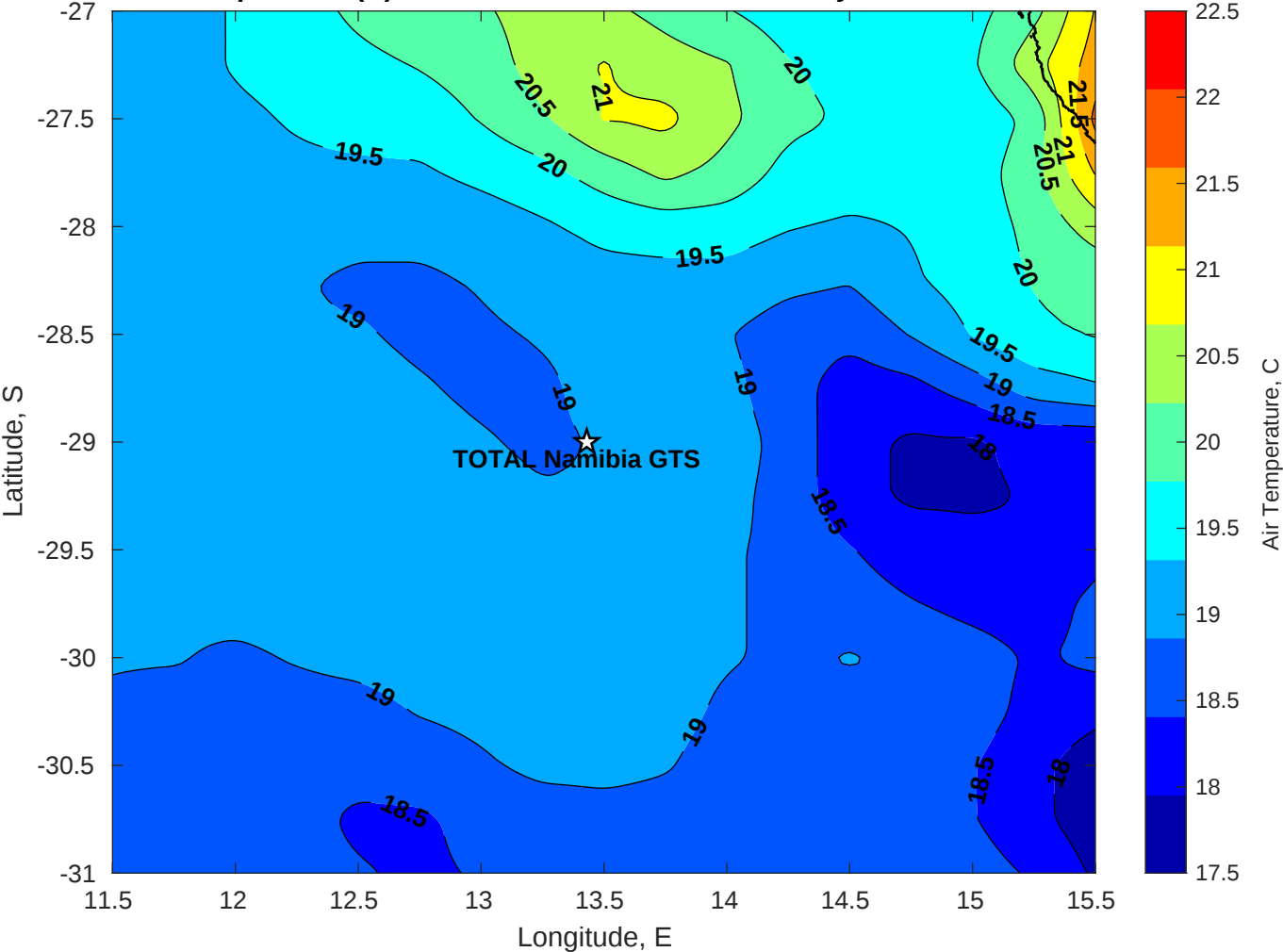
Air Temperature (C) for TOTAL Namibia GTS at 22-May-2025
