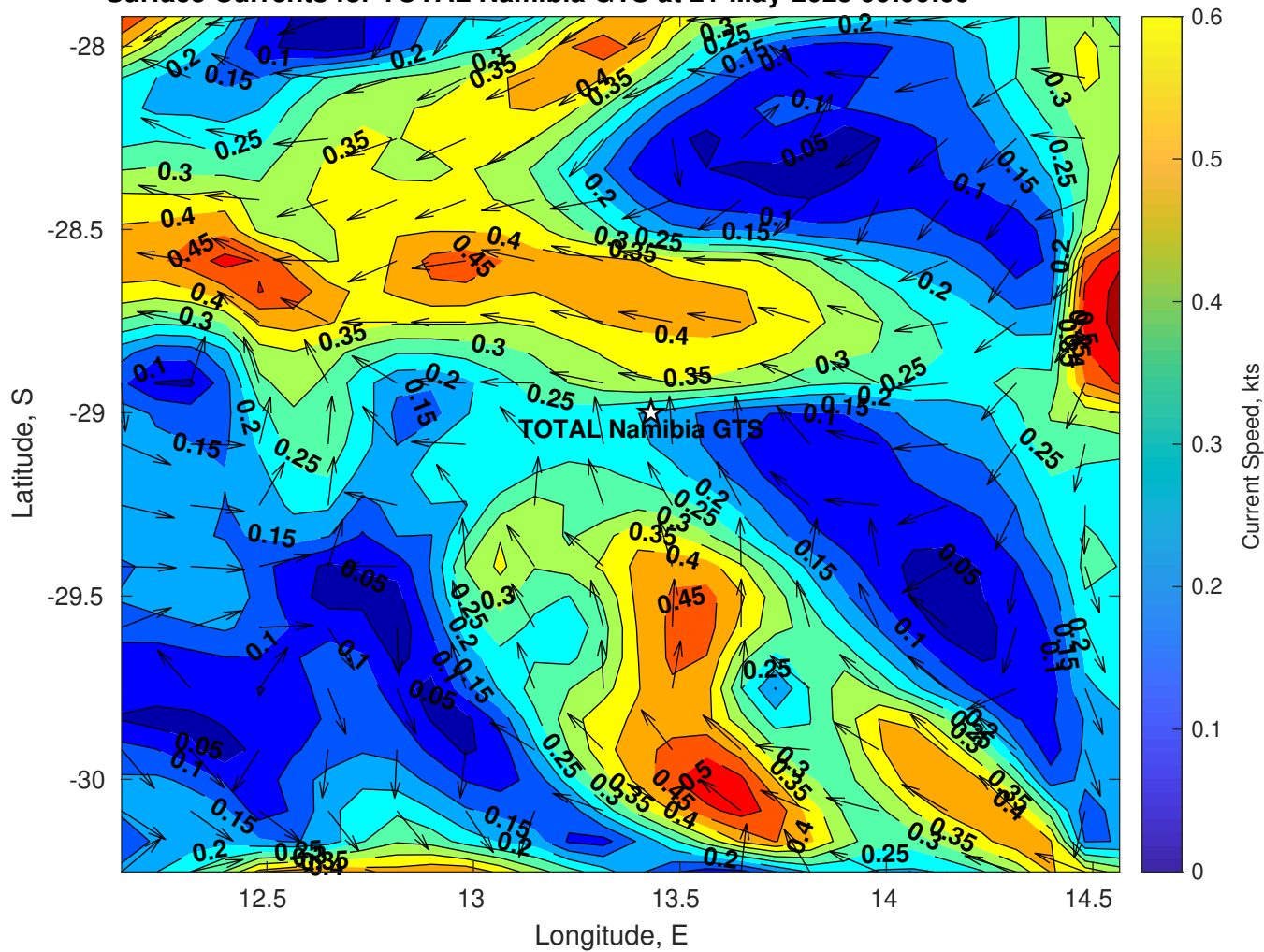
Surface Currents for TOTAL Namibia GTS at 21-May-2025 00:00:00
