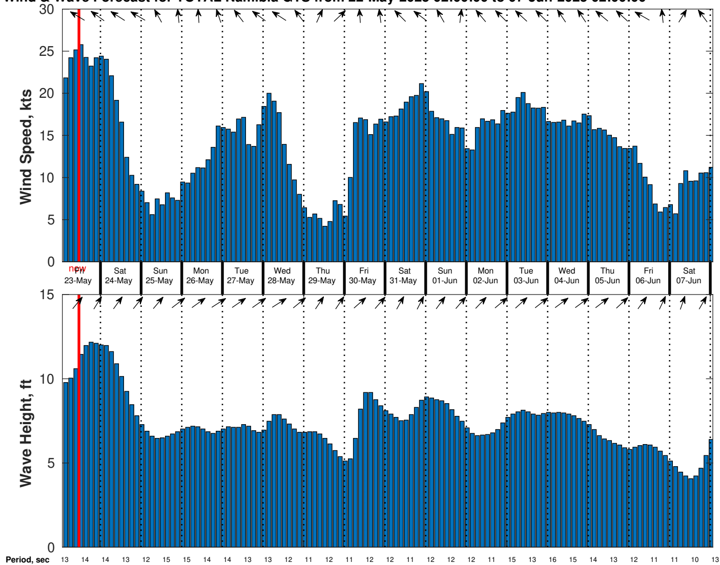
Wind & Wave Forecast for TOTAL Namibia GTS from 22-May-2025 02:00:00 to 07-Jun-2025 02:00:00
