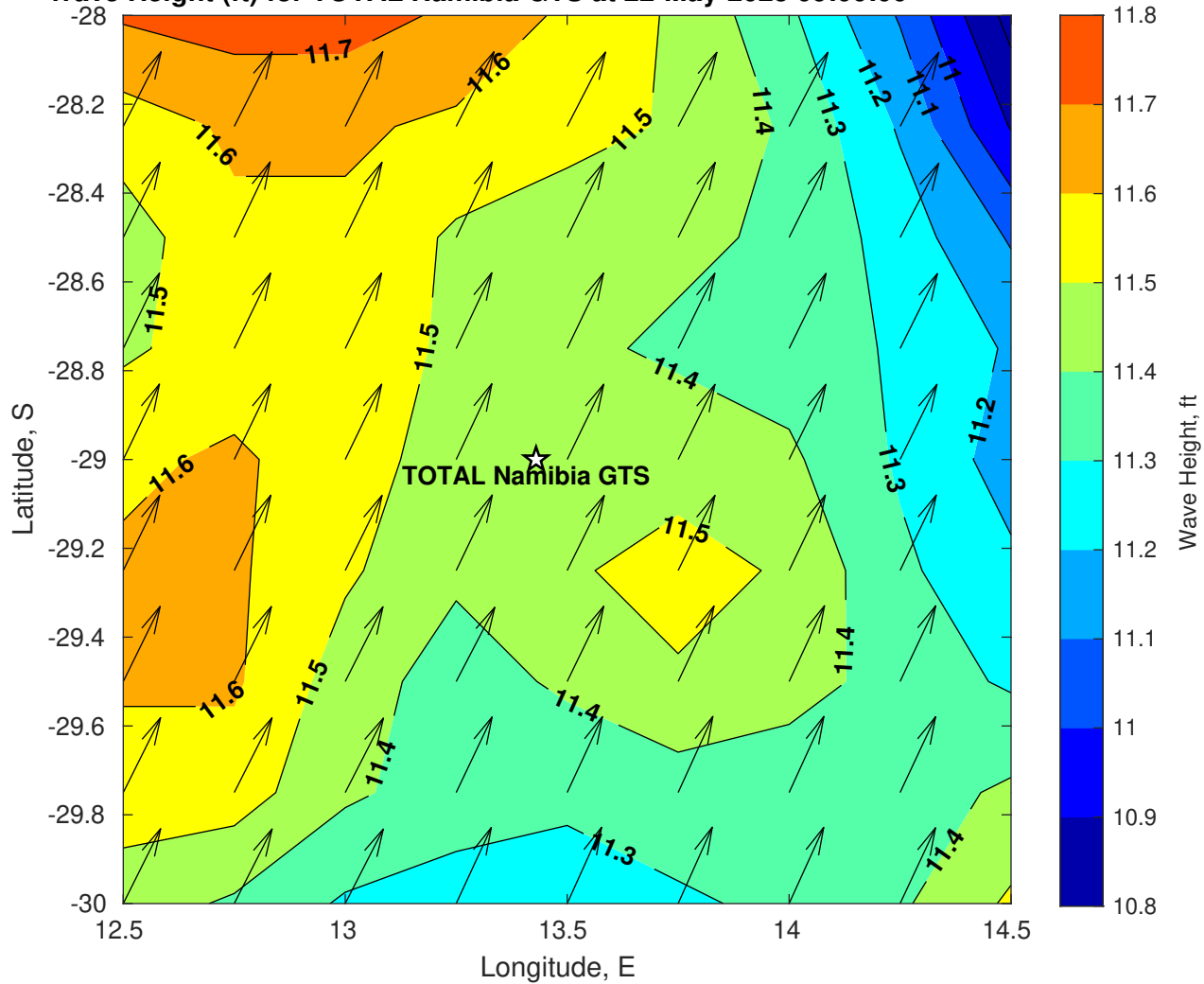
Wave Height (ft) for TOTAL Namibia GTS at 22-May-2025 09:00:00
