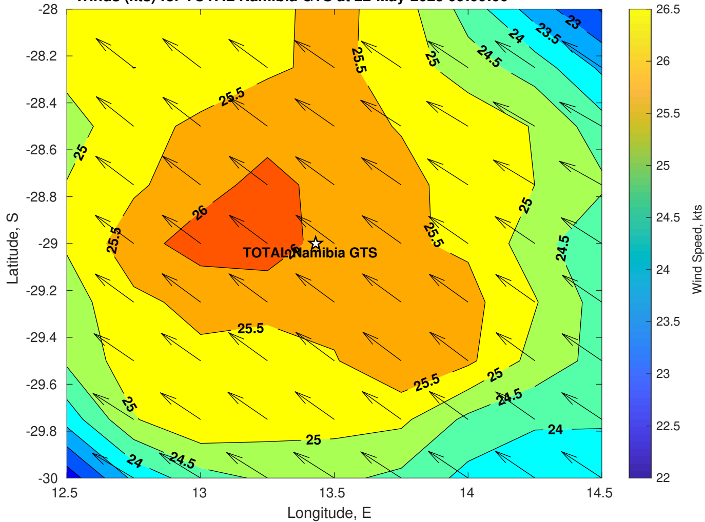
Winds (kts) for TOTAL Namibia GTS at 22-May-2025 09:00:00
