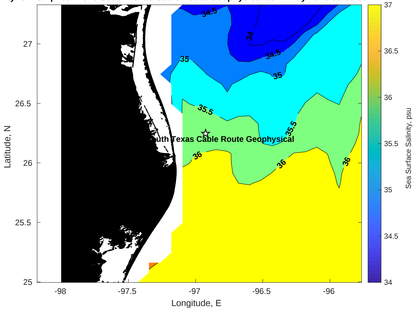
Surface Salinity for Tampnet P2378 South Texas Cable Route Geophysical at 21-May-2025 00:00:00
