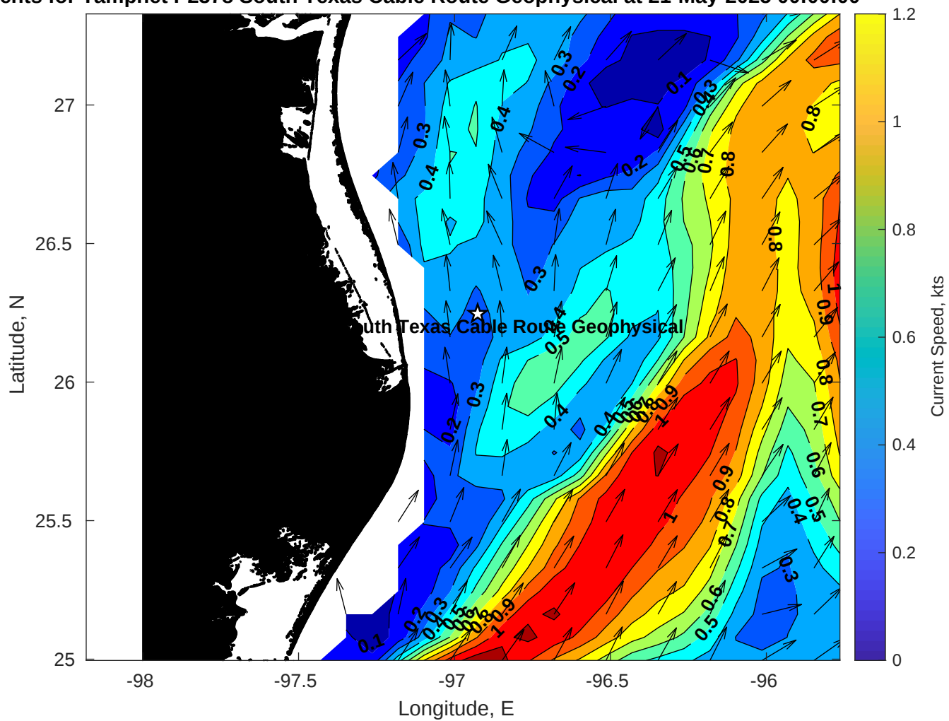
Surface Currents for Tampnet P2378 South Texas Cable Route Geophysical at 21-May-2025 00:00:00
