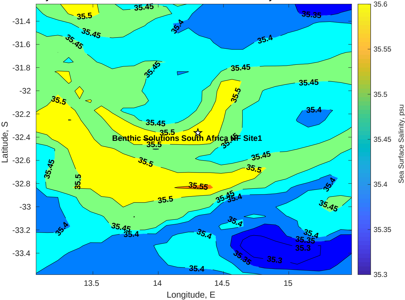
Surface Salinity for Benthic Solutions South Africa HF Site1 at 22-May-2025 00:00:00
