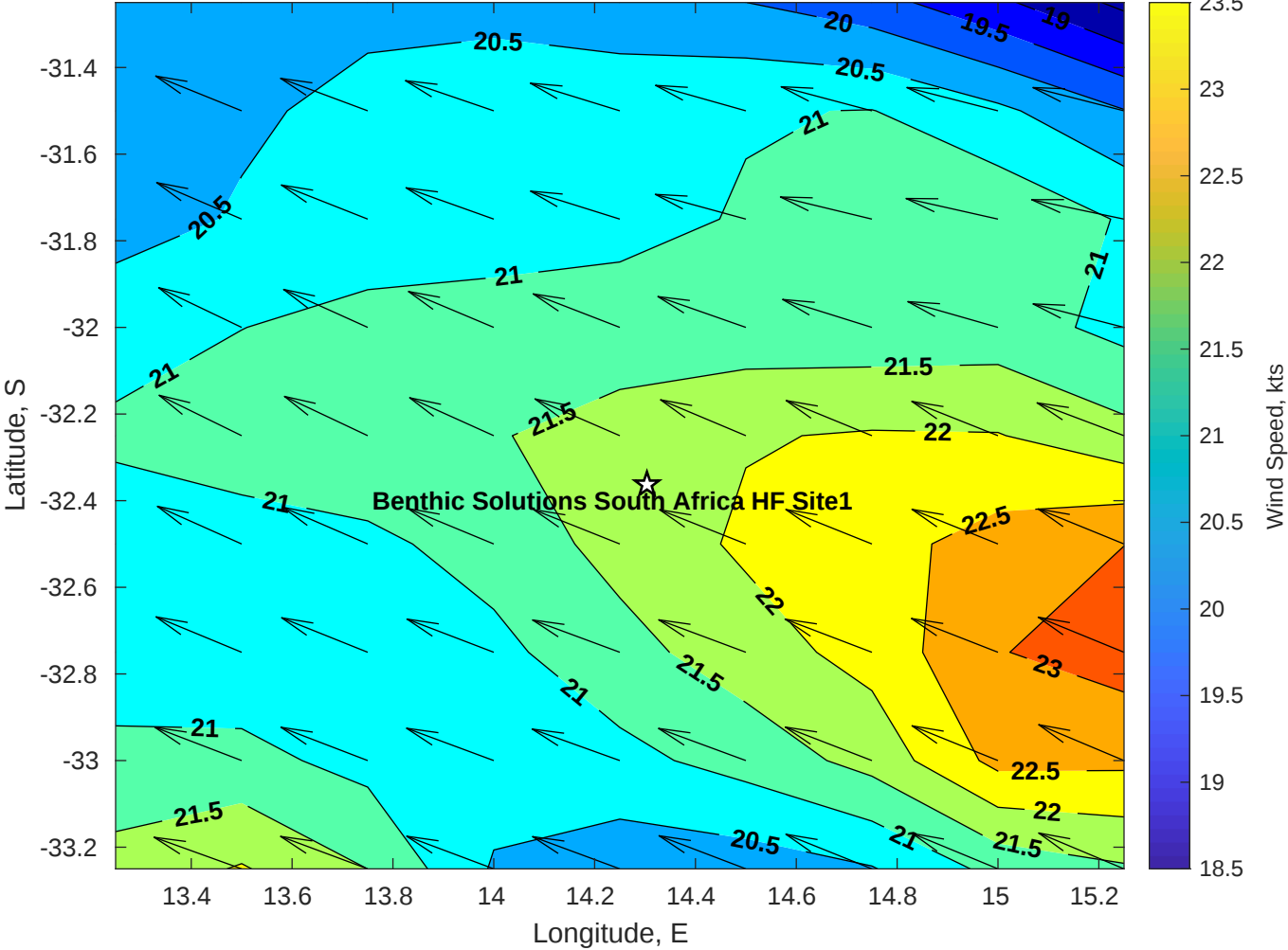
Winds (kts) for Benthic Solutions South Africa HF Site1 at 23-May-2025 09:00:00
