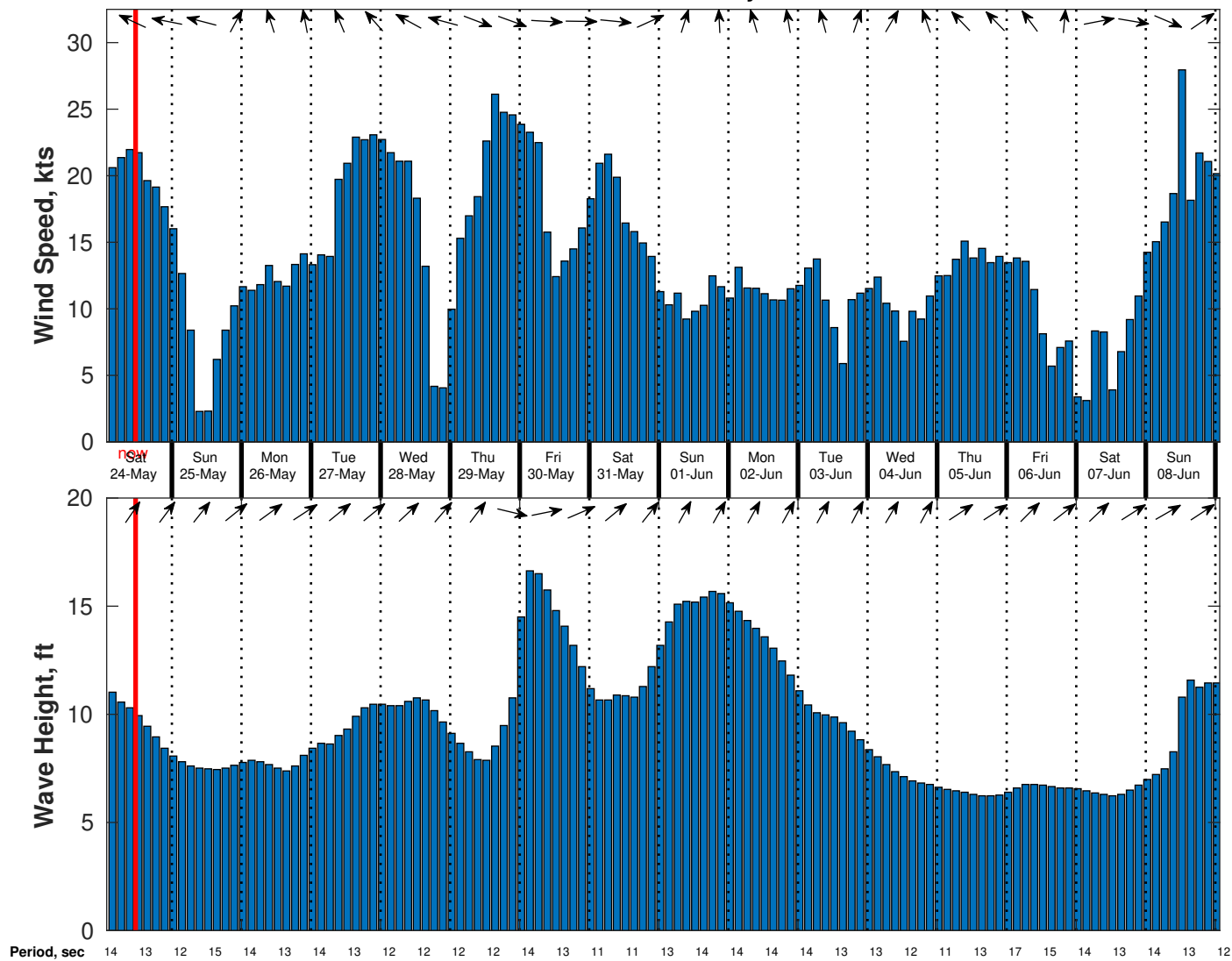
Wind & Wave Forecast for Benthic Solutions South Africa HF Site1 from 23-May-2025 02:00:00 to 08-Jun-2025 02:00:00
