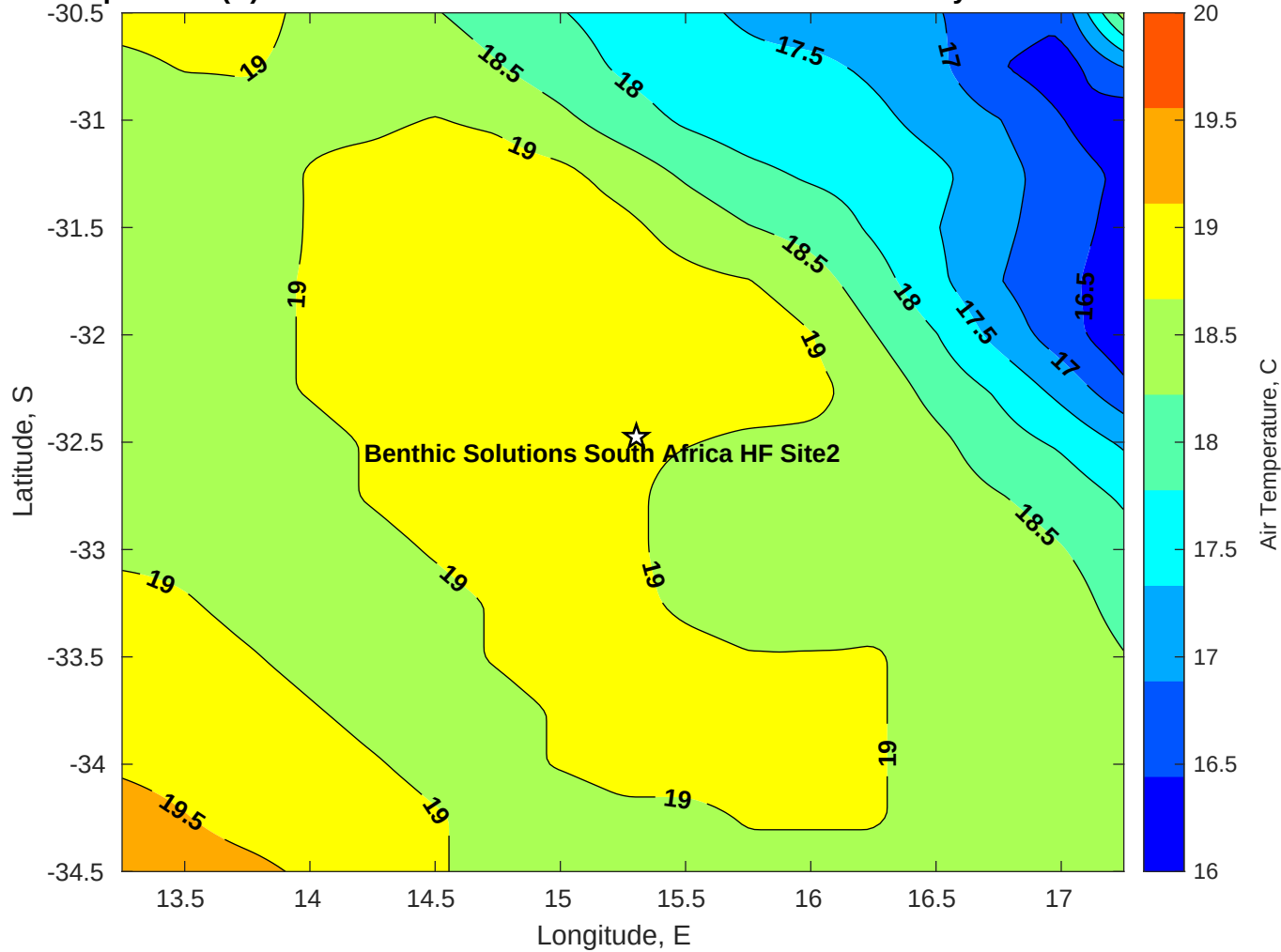
Air Temperature (C) for Benthic Solutions South Africa HF Site2 at 23-May-2025
