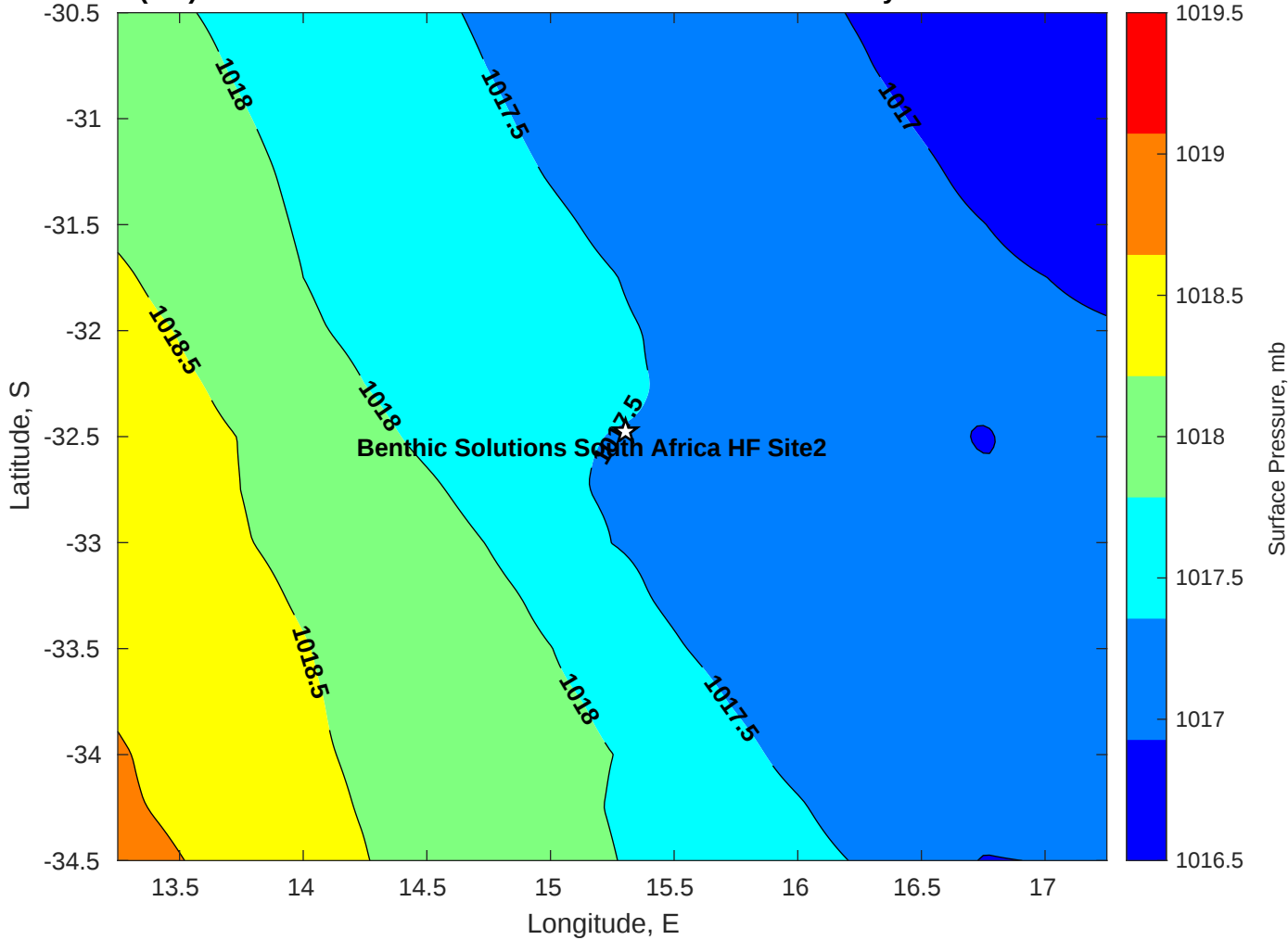
Surface Pressure (mb) for Benthic Solutions South Africa HF Site2 at 25-May-2025 00:00:00
