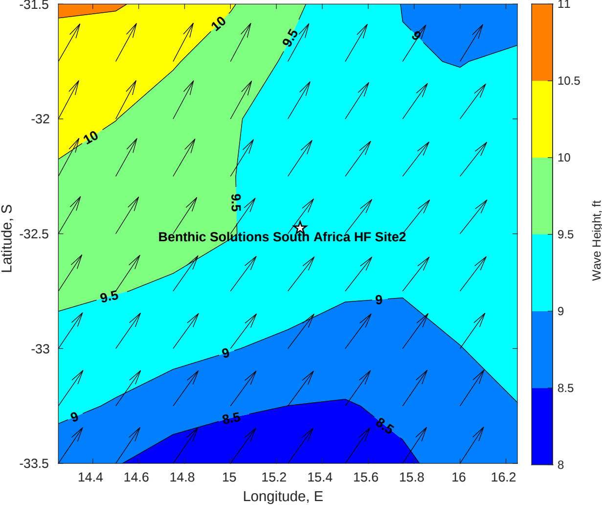
Wave Height (ft) for Benthic Solutions South Africa HF Site2 at 23-May-2025 09:00:00
