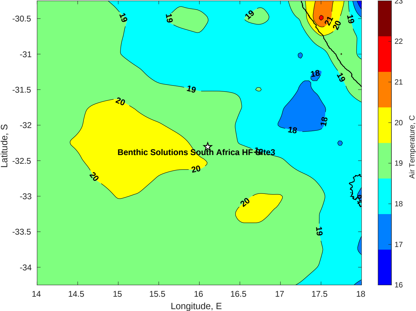
Air Temperature (C) for Benthic Solutions South Africa HF Site3 at 23-May-2025
