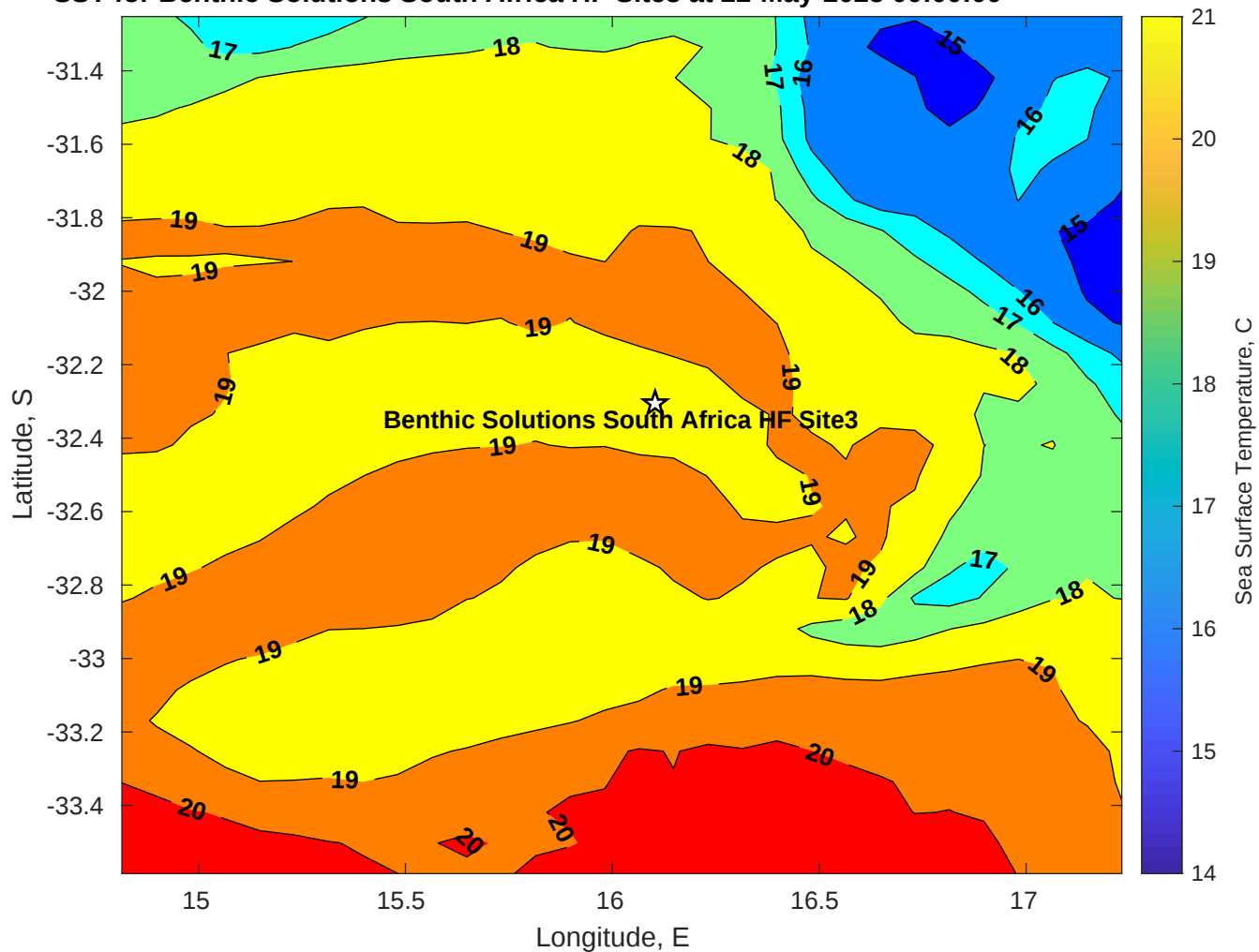
SST for Benthic Solutions South Africa HF Site3 at 22-May-2025 00:00:00
