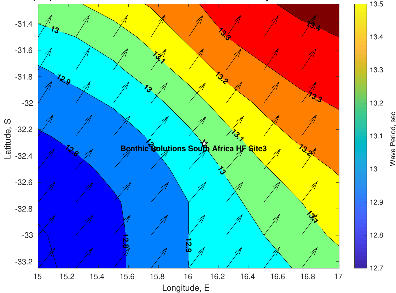
Wave Period (sec) for Benthic Solutions South Africa HF Site3 at 23-May-2025 09:00:00
