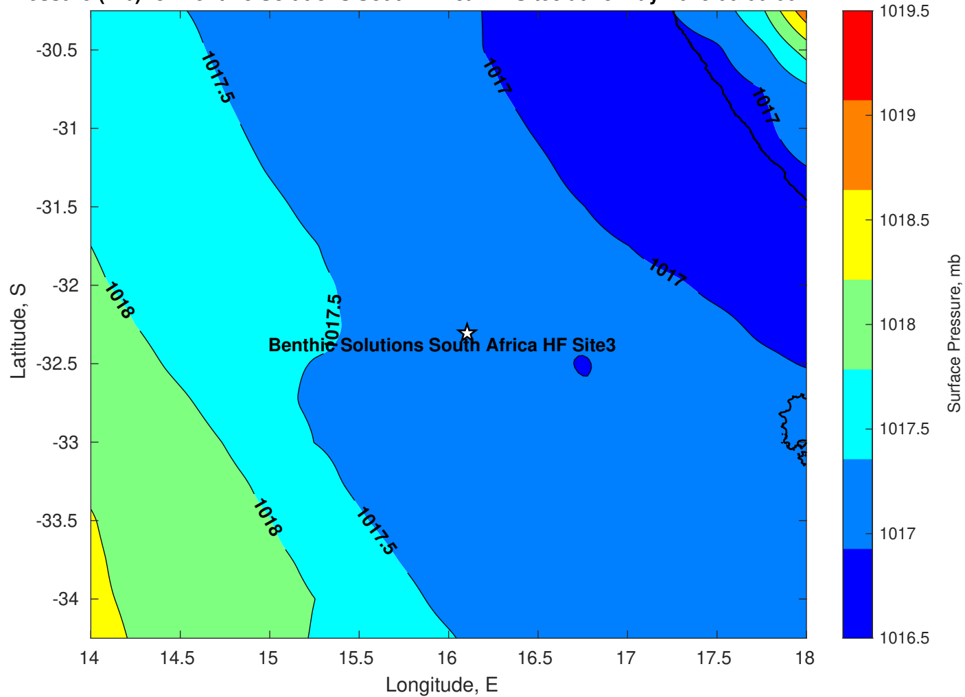
Surface Pressure (mb) for Benthic Solutions South Africa HF Site3 at 25-May-2025 00:00:00
