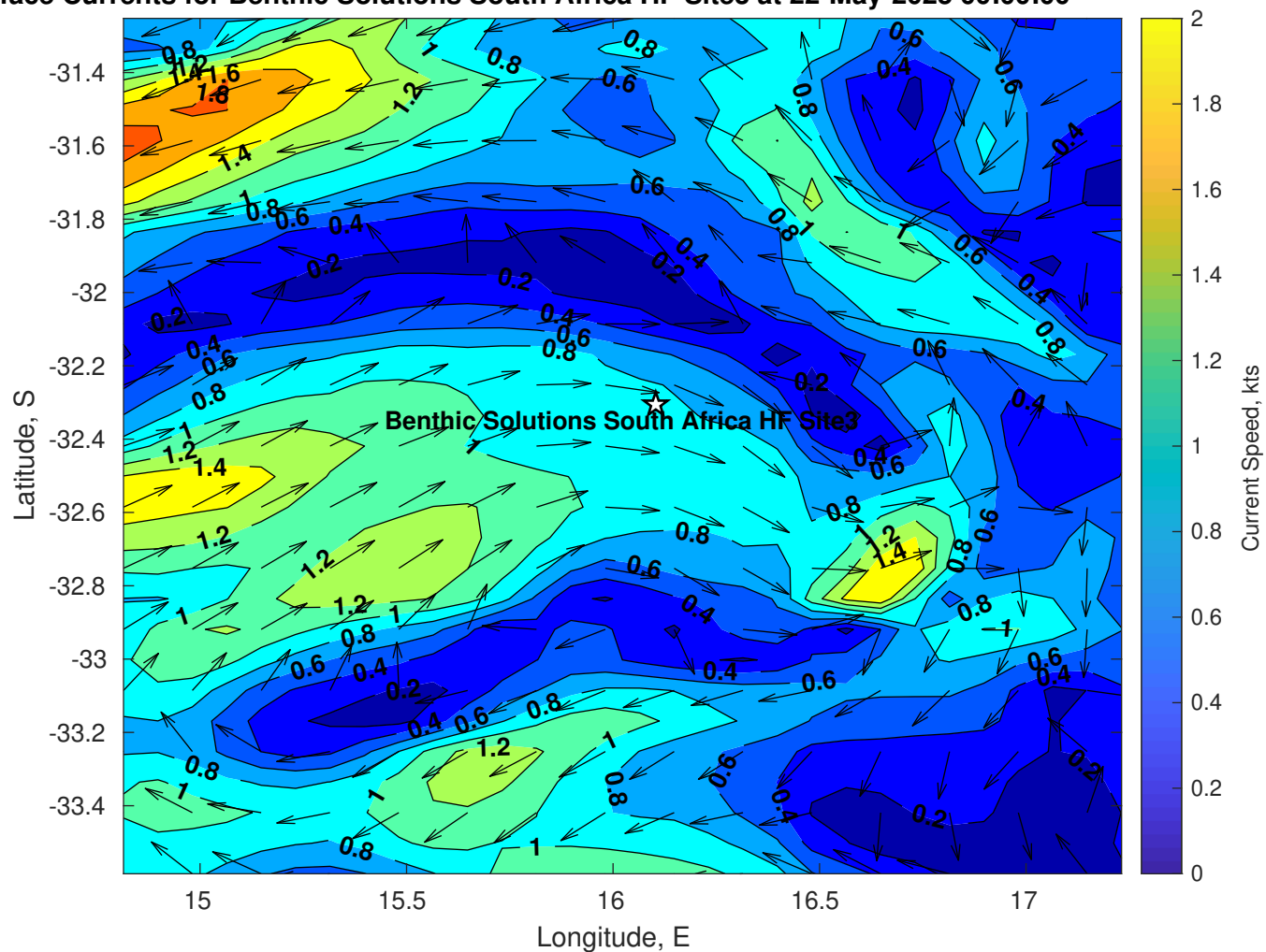
Surface Currents for Benthic Solutions South Africa HF Site3 at 22-May-2025 00:00:00
