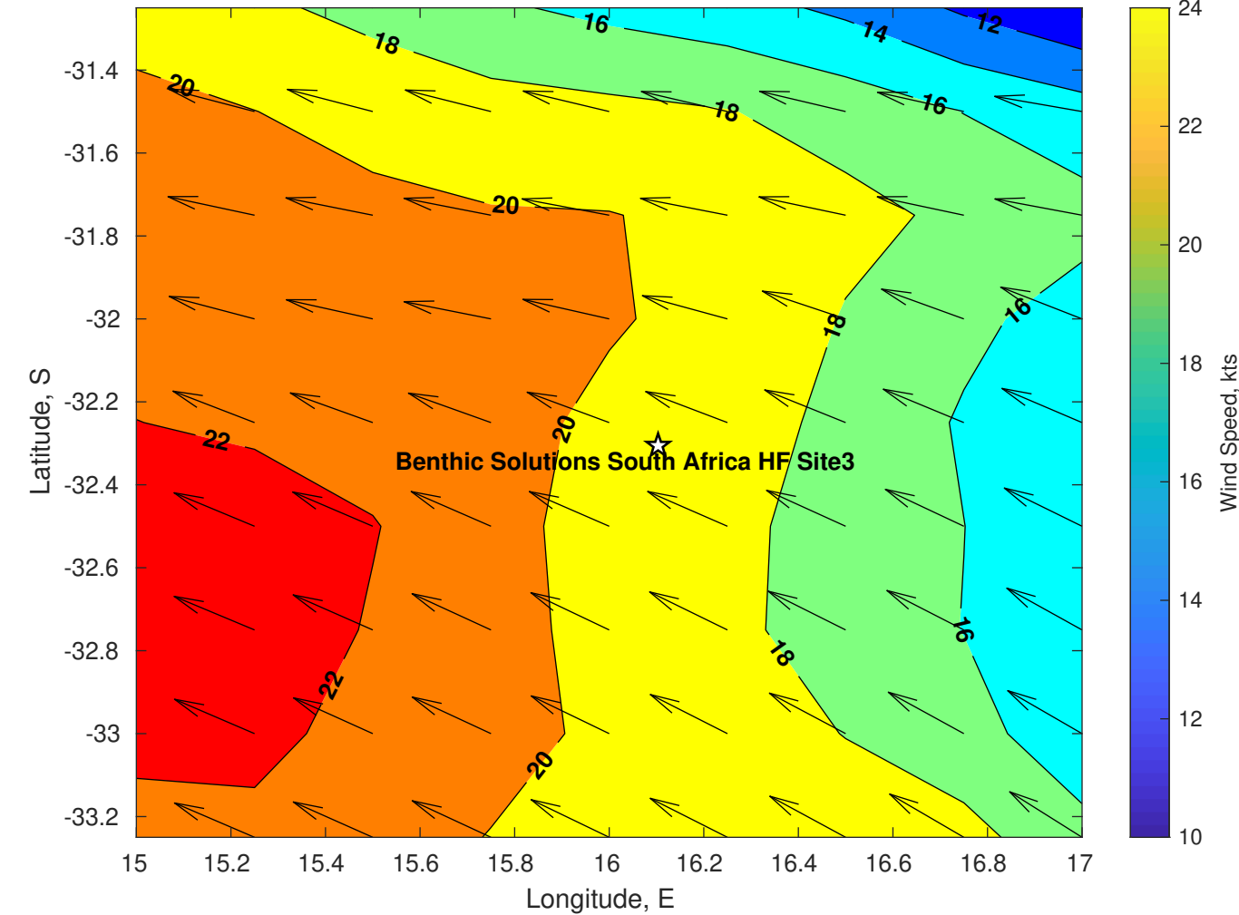
Winds (kts) for Benthic Solutions South Africa HF Site3 at 23-May-2025 09:00:00
