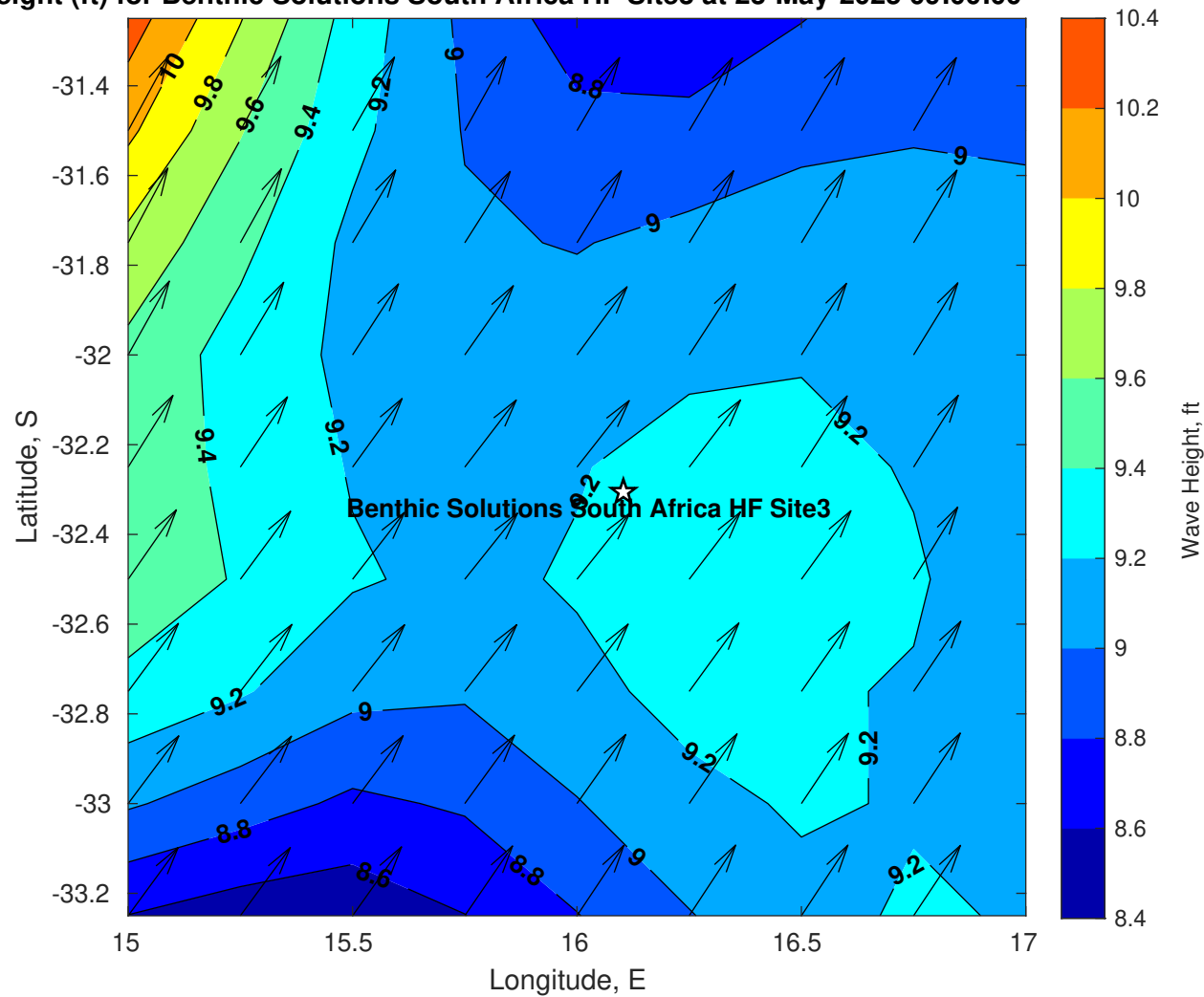
Wave Height (ft) for Benthic Solutions South Africa HF Site3 at 23-May-2025 09:00:00
