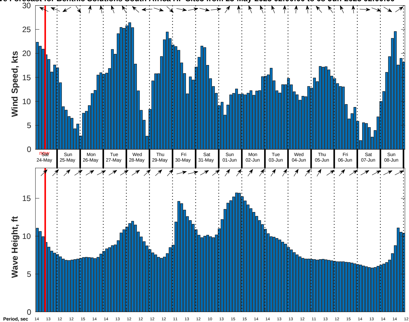
Wind & Wave Forecast for Benthic Solutions South Africa HF Site3 from 23-May-2025 02:00:00 to 08-Jun-2025 02:00:00
