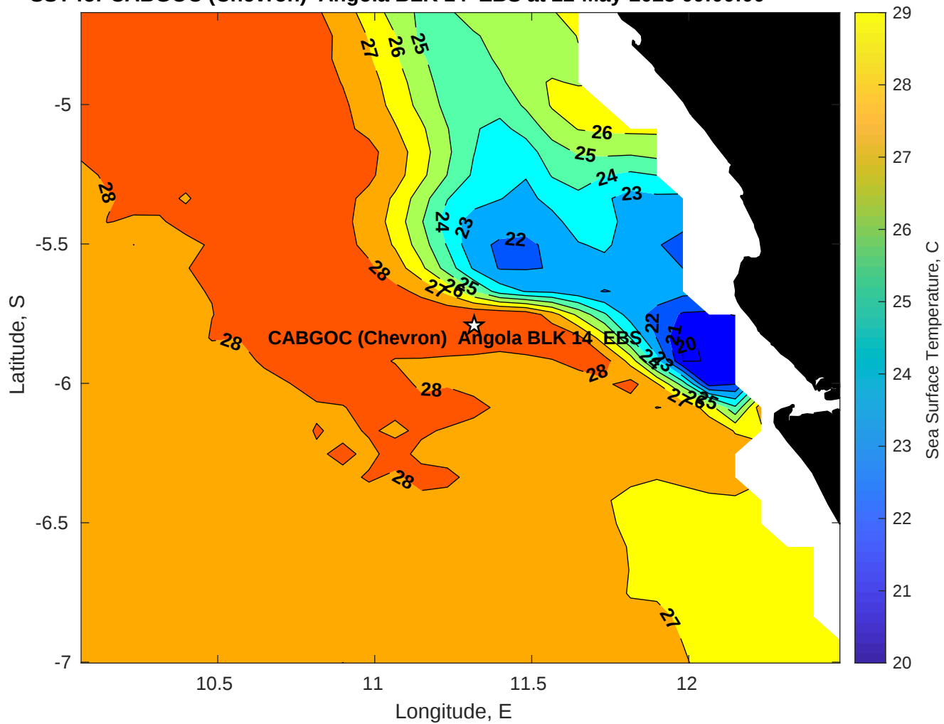
SST for CABGOC (Chevron) Angola BLK 14 EBS at 22-May-2025 00:00:00
