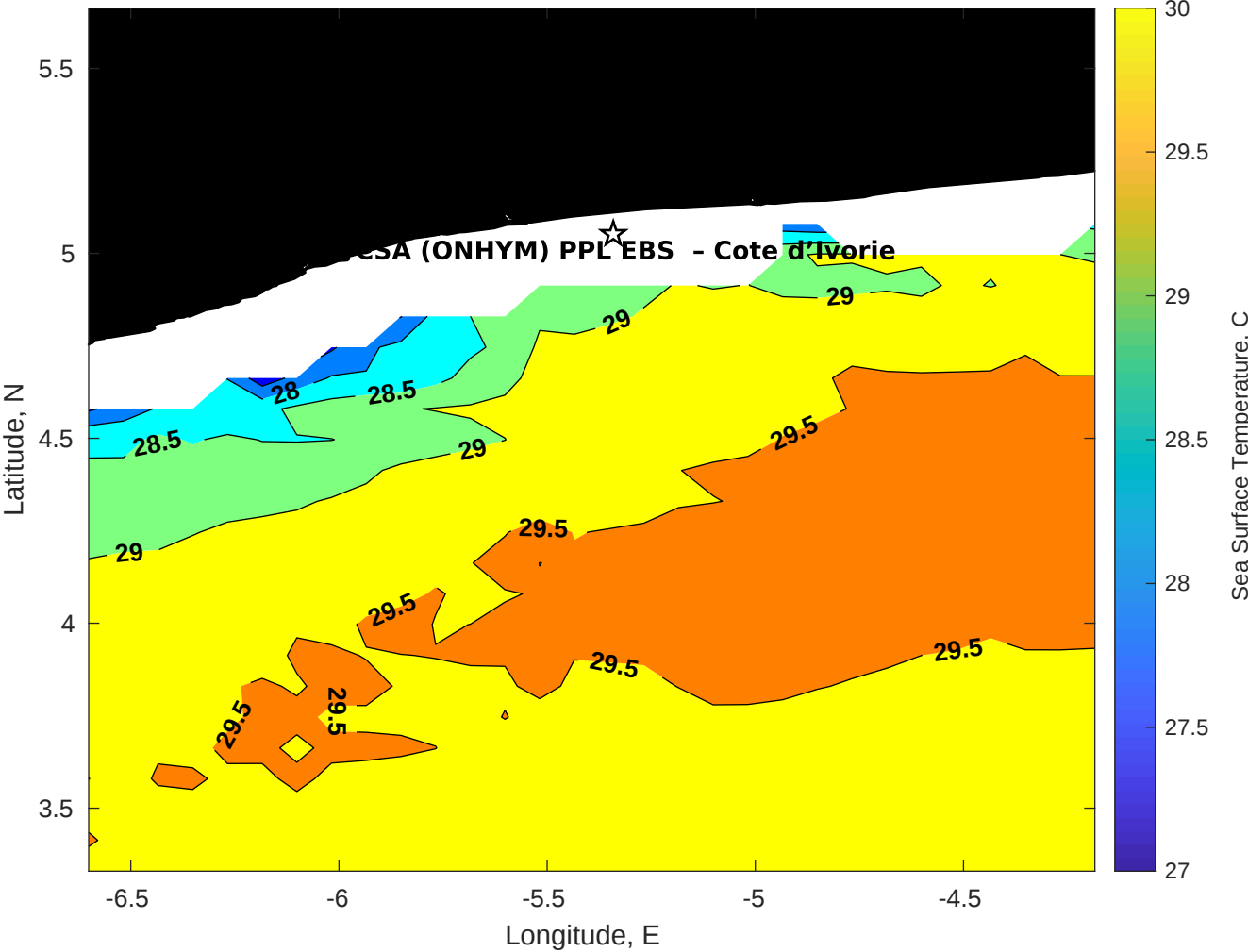
SST for CSA (ONHYM) PPL EBS - Cote d'Ivoire at 22-May-2025 00:00:00
