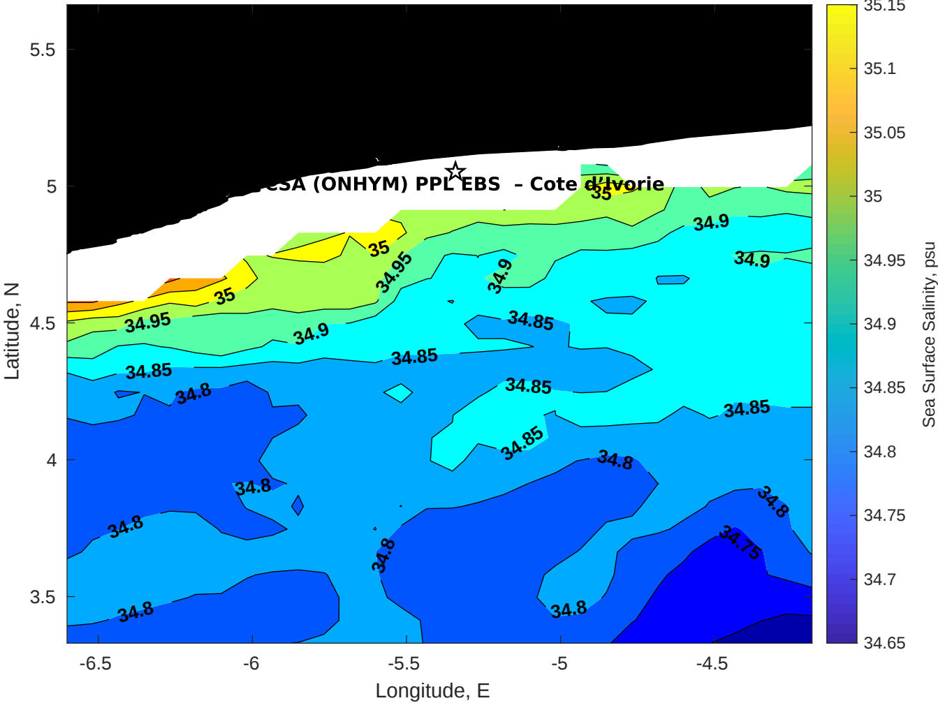
Surface Salinity for CSA (ONHYM) PPL EBS - Cote d'Ivoire at 22-May-2025 00:00:00
