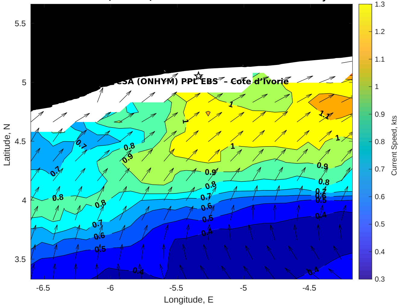
Surface Currents for CSA (ONHYM) PPL EBS - Cote d'Ivoire at 22-May-2025 00:00:00
