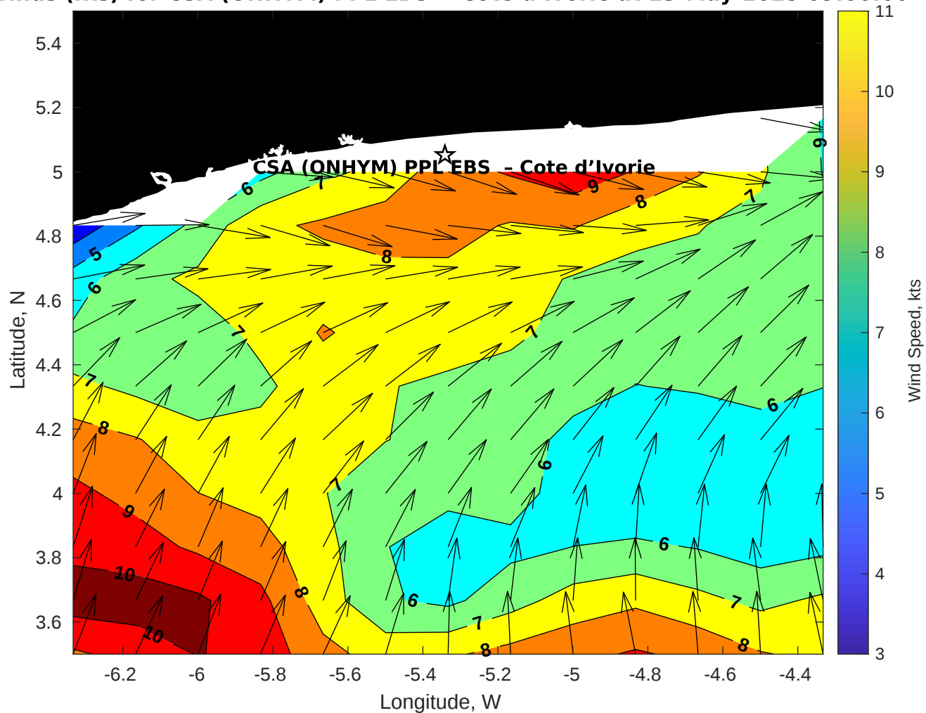
Winds (kts) for CSA (ONHYM) PPL EBS - Cote d'Ivoire at 23-May-2025 09:00:00
