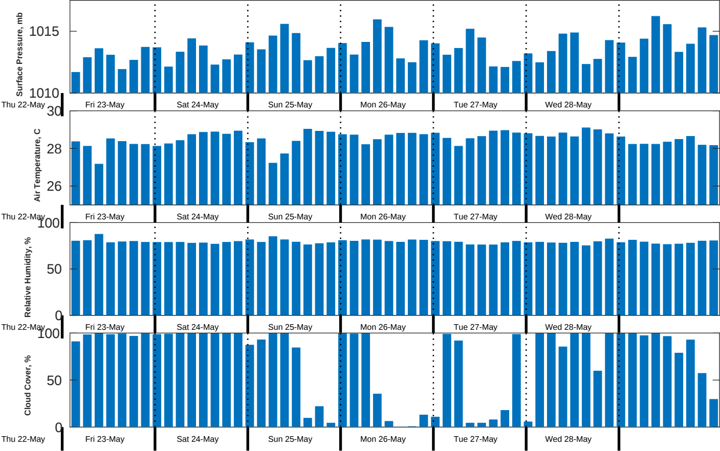
Met Forecast for CSA (ONHYM) PPL EBS - Cote d'Ivoire from 23-May-2025 00:00:00 to 30-May-2025 00:00:00
